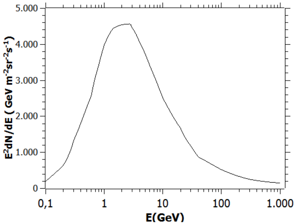
Figure 2: The previous figure is replotted to allow the calculation of the number-flux as a function of energy. Integration displays the accumulation of protons below 3 GeV, in search of a relaxed configuration.
