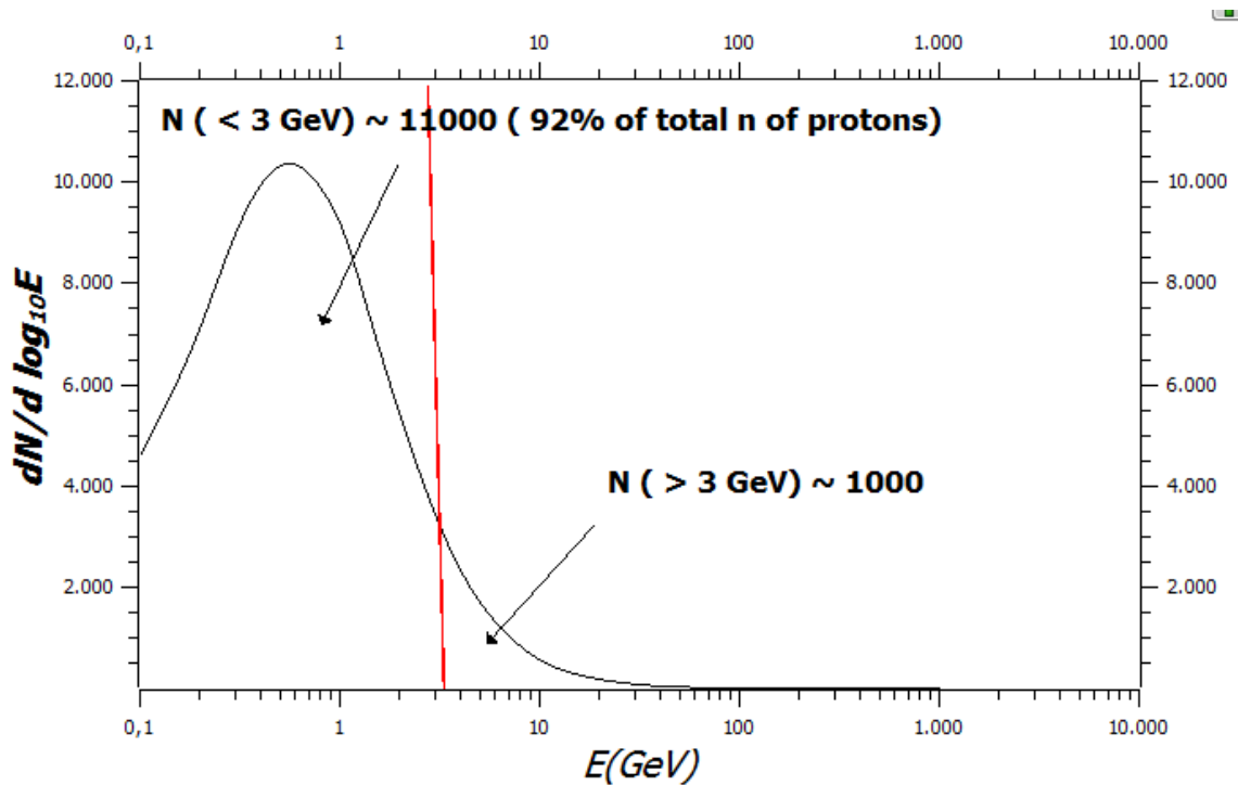
Figure 2: The previous figure is replotted to allow the calculation of the number-flux as a function of energy. Integration displays the accumulation of protons below 3 GeV, in search of a relaxed configuration.
