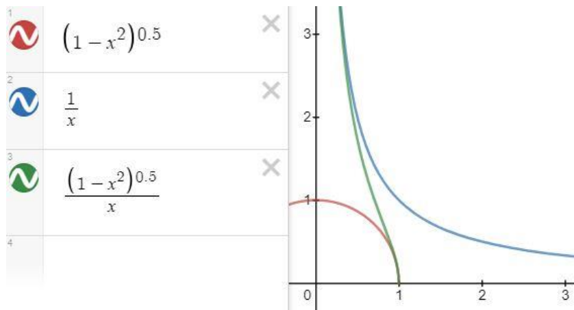
Figure 8: The 1/\gamma , 1/\beta and 1/\gamma\beta graphs 87
