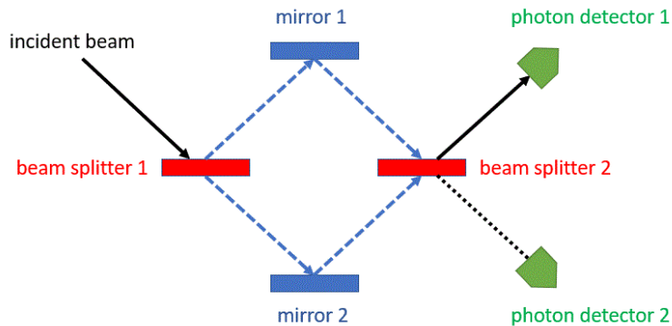
Figure 9: The Mach-Zehnder interferometer
