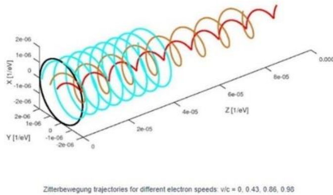
Figure 11: The Compton radius must decrease with increasing velocity
