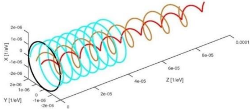
Zitterbewegung trajectories for different electron speeds: v/c = 0, 0.43, 0.86, 0.98
