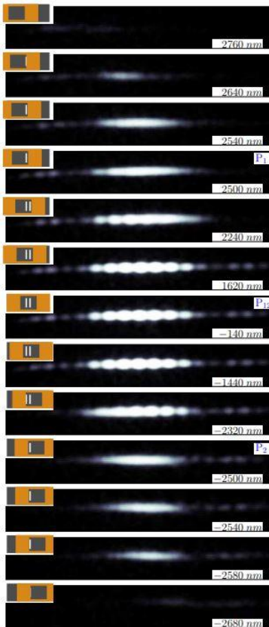
Figure 5: Diffraction and interference patterns (double-slit experiment with electrons) 83
