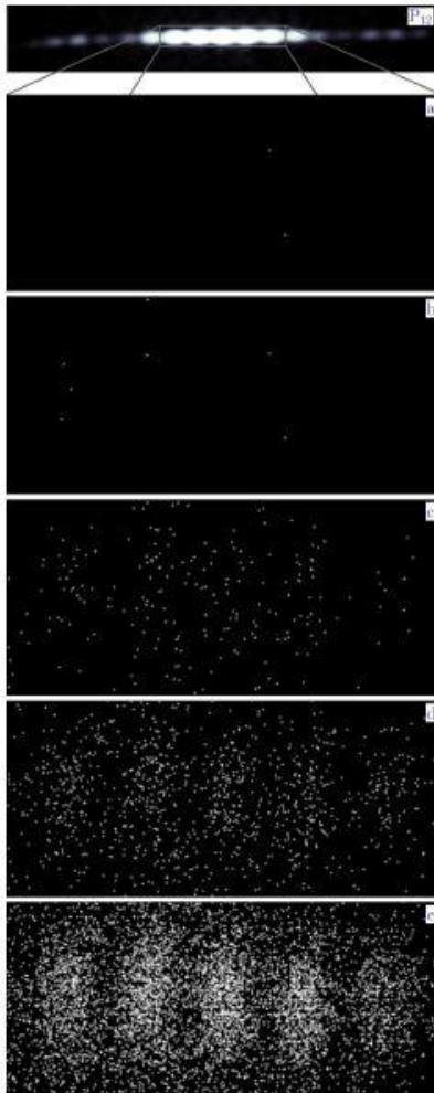
Figure 6: Diffraction and interference patterns (double-slit experiment with electrons) 84
