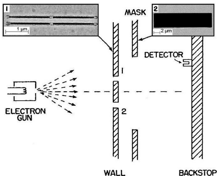
Figure 4: The actual double-slit experiment with electrons 82
