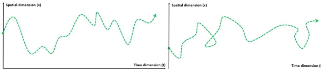
Figure 2: A well- and a not-well behaved trajectory in spacetime 29
