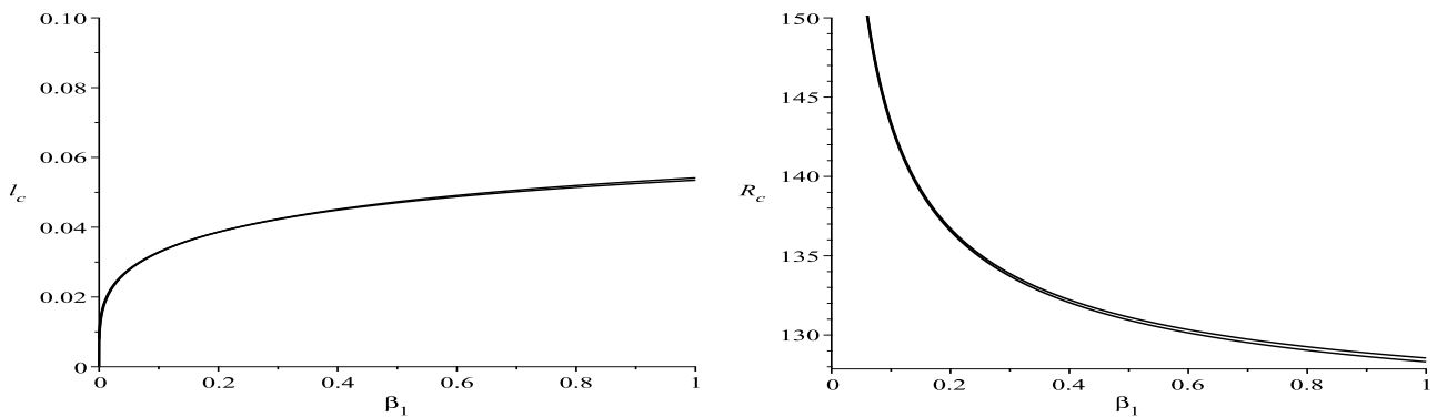
Figure 6: (left) Plots of l_c vs \beta_1 , linear (top) and nonlinear (bottom). (right) Plots of R_c vs \beta_1 , linear (bottom) and nonlinear (top). Here D' = U' = H' = 1 , \gamma_1 = 1/20000 , \gamma_2 = 1/10000 , \gamma_3 = \gamma_4 = 0 , S = 100 , \beta_2 = 0 , and \tau = 1/10 .
