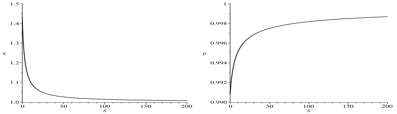
Figure 5: (left) Plots of \kappa vs S . (right) Plots of \rho vs S . Here D' = U' = H' = 1 , \gamma_1 = 1/20000 , \gamma_2 = 1/10000 , \gamma_3 = \gamma_4 = 0 , \beta_1 = 1 , \beta_2 = 0 , and \tau = 1/10 .
