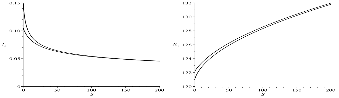
Figure 4: (left) Plots of l_c vs S , linear (top) and nonlinear (bottom). (right) Plots of R_c vs S , linear (bottom) and nonlinear (top). Here D' = U' = H' = 1 , \gamma_1 = 1/20000 , \gamma_2 = 1/10000 , \gamma_3 = \gamma_4 = 0 , \beta_1 = 1 , \beta_2 = 0 , and \tau = 1/10 .
