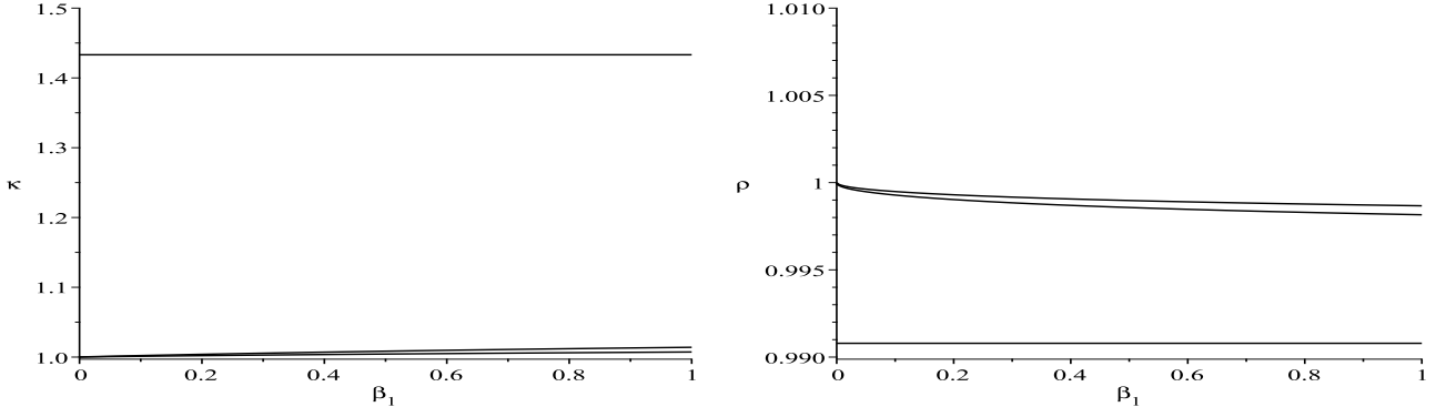
Figure 7: (left) Plots of \kappa vs \beta_1 . (right) Plots of \rho vs \beta_1 . Here D' = U' = H' = 1 , \gamma_1 = 1/20000 , \gamma_2 = 1/10000 , \gamma_3 = \gamma_4 = 0 , S \in \{0, 100, 200\} , \beta_2 = 0 , and \tau = 1/10 .
