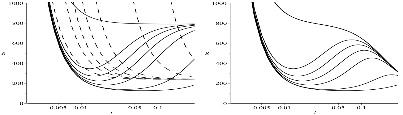
Figure 8: (left) Figure 3 of Cox & Leibovich (1993). (right) nonlinear steady states R vs l . Here D' = U' = H' = 1 , S = 100 , \gamma_1 = 1/40000 , \gamma_2 = -\gamma_3 = -\gamma_4 = 1/20000 , \beta_1 = -\beta_2 \in [1/20000, 1/2] , and \tau = 10/67 .
