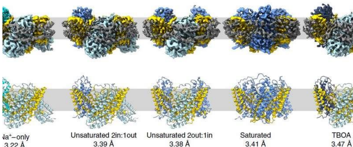
Figure 2. The structure of the glutamate transporter from archaea in different states. Each picture represents a snapshot in which protomers are presented in the following states: inward open (steel blue), intermediate-outward occluded apo (cyan), intermediate-outward occluded Asp (cornflower blue), outward-open TBOA (dark blue) Credit: Valentina Arkhipova et al./Nature Communications
