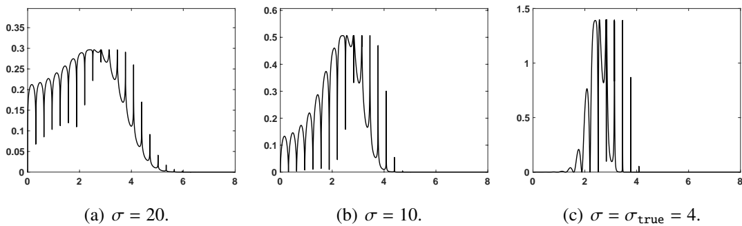
Figure 1: Conditional posteriors corresponding to different values of \sigma : (a) \sigma = 20 , (b) \sigma = 10 , (c) \sigma = \sigma_{\text{true}} = 4 .
