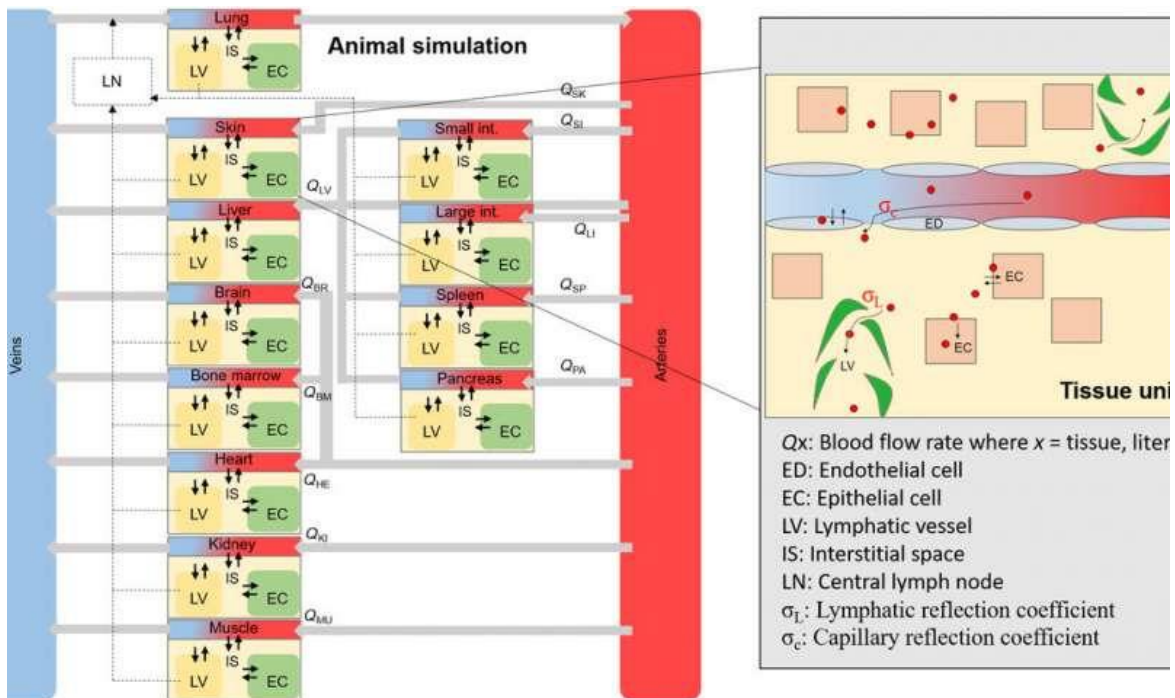
An overall schematic of the animal NM simulation. Scheme of the overall tissue and blood compartments that make up the full animal. Each tissue compartment is interconnected through blood flow rates and contains sub-compartments (zoomed-in area), where an NM will distribute upon internalization through endothelial fenestrae. Credit: Science Advances , doi: 10.1126/sciadv.aax2642
