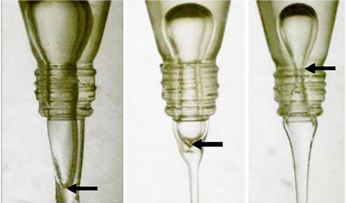
Formation of encapsulated bubbles Credit: Lokesh Rohilla
