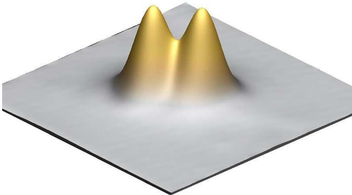
Figure 2: An image of two titanium atoms positioned just 1 nanometer apart and used to perform complex quantum operations. Credit: IBM
