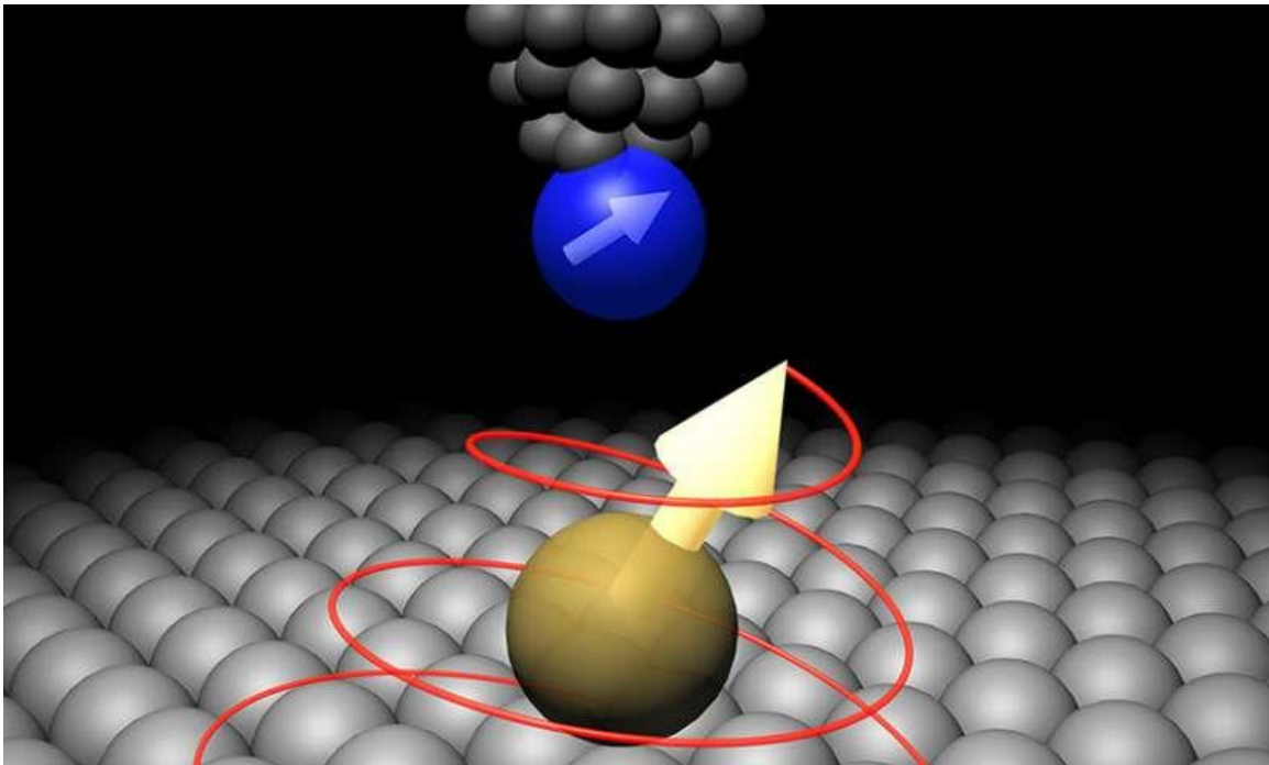
Figure 1: An artist's view of the quantum dance of a single titanium atom (yellow ball) sitting atop a specially prepared surface of magnesium oxide. The top of the image shows the STM's sharp needle tip, which is used to perform coherent control. Credit: IBM
