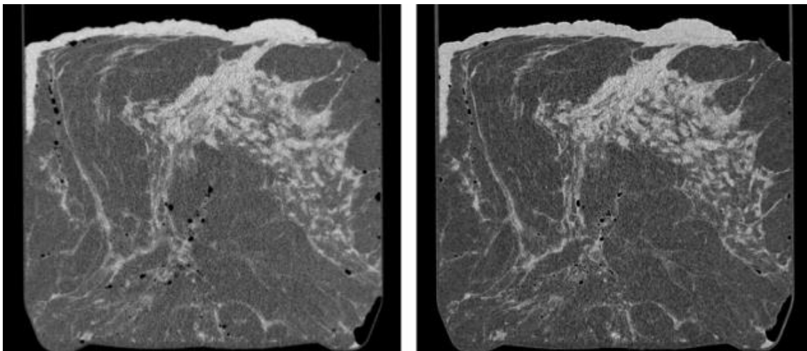
Absorption-based CT (left) and propagation-based phase-contrast CT (right) of a breast mastectomy sample, both using a dose of 4 mGy. (Courtesy: Seyedamir Tavakoli Taba)
