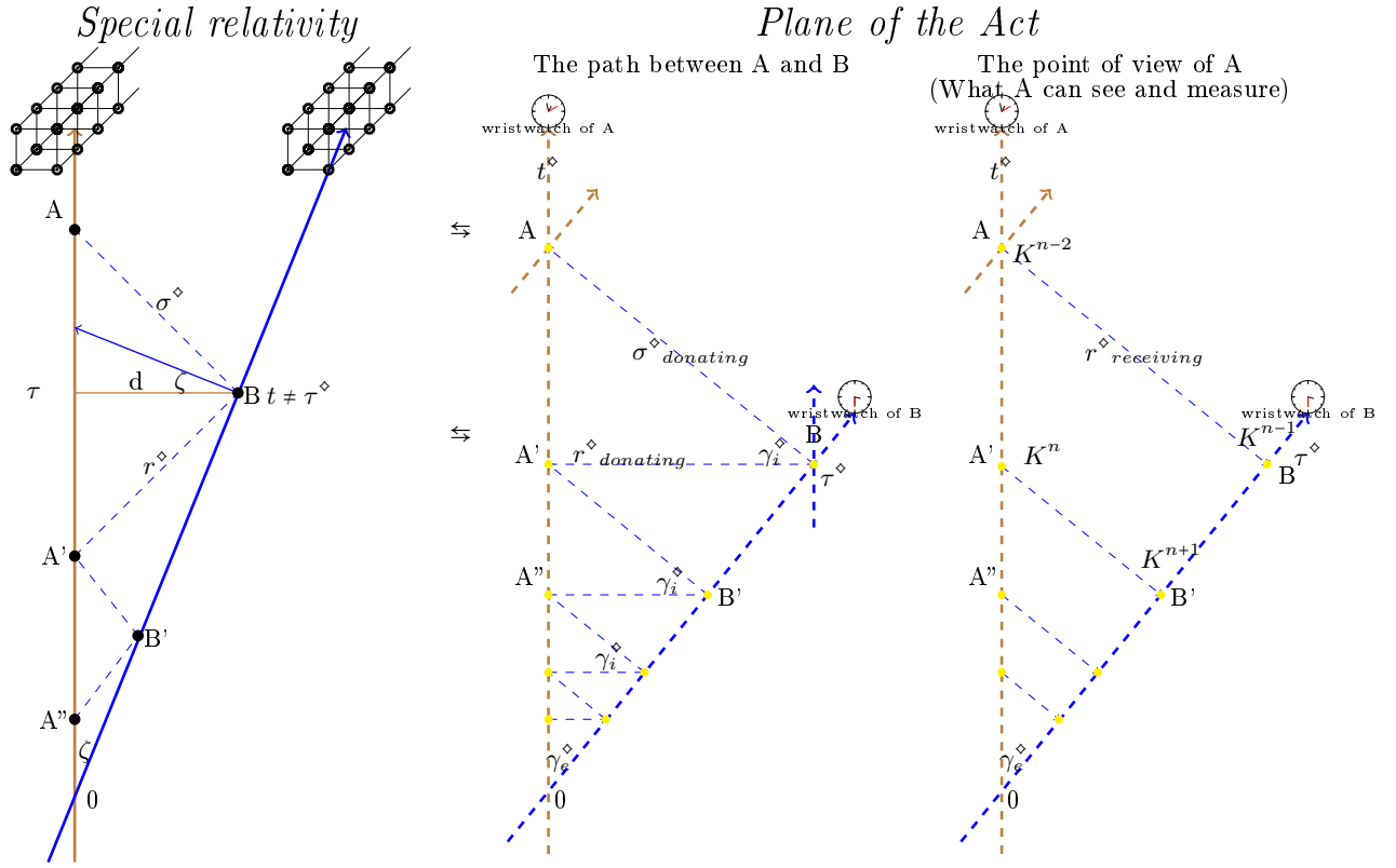
Figure 5. isomorphism: the representation of the temporal and spatial distances between the real points A, B, A', B', A'', B'', \dots in the Minkowski spacetime, on the left, is equivalent to the representation in the Intention historical plane, on the right, with the conversion v = \tanh \zeta \rightarrow V = 1 - \cos \gamma^\diamond and e^{-\zeta} = \cos \gamma^\diamond . The difference is that while the Intention historical plane defines only these points as the unique real, and the spatial distances, therefore, represent the correspondence between t^\diamond and \tau^\diamond that are therefore joined instantly at every act of donation/receiving, the Minkowski spacetime defines all the intermediate points too (that are in potency and therefore not real in the intention) and establishes a correspondence between each point on t axis and \tau axis (be it real or imaginary) making the speed of light finite and traveling in the spacetime. As it is shown in (Peluso 13 jan 2019 [77]) the Intention historical plane is the primitive space where General Theory of Relativity and Quantum Mechanics are reconciled.
