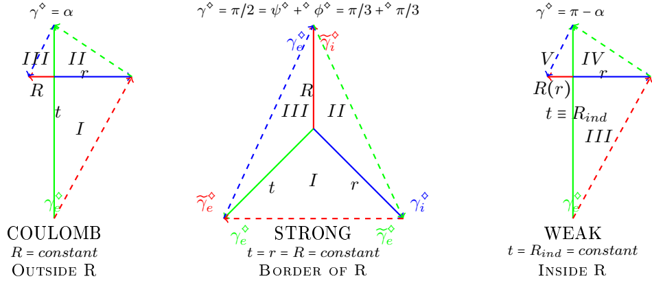
The three configurations of the spacetime of the relationship
