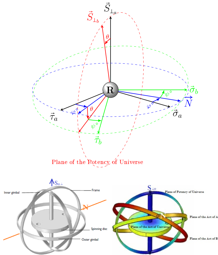
Figure 12. weaving: Since the sole universe thread is sequential, without loops, the time axes of different individuals never intersect each other, but they must respect a minimum weaving distance equal to their radius R . Therefore, the two reference frames must moreover weave around the axis of the nodes r forming the two angles of weaving \vartheta_a and \vartheta_b where \vartheta_a^\diamond + \vartheta_b^\diamond = \vartheta
