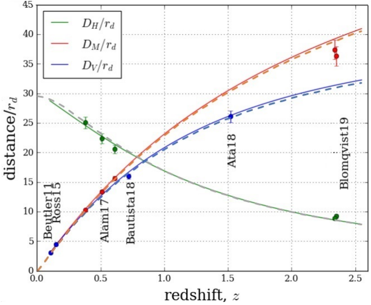
Figure 23. BAO measurement (Agathe VS. et al. 2019 [66] ) of D_H/r_d and D_M/r_d using BOSS galaxies (Alam et al. 2017), Ly\alpha absorption in BOSS-eBOSS quasars (Agathe et al. 2019) and correlation between BOSS-eBOSS quasars and Ly\alpha absorption (Blomqvist et al. 2019). Other measurements give D_V/r_d , with D_V = D_M^{2/3}(zD_H)^{1/3} , using galaxies (Beutler et al. (2011), Ross et al. (2015), Bautista et al. (2018)) and BOSS-eBOSS quasars (Ata et al.2018). Solid lines show the \Lambda CDM values (Planck Collaboration et al.2016). These can be compared to the correspondingly colored lines, which represents predictions of the fiducial Planck \Lambda CDM model (with m = 0.3183 , h = 0.6704 ) and the prediction of the Intention model (dashed lines) when r_{s_{drag}} = 101.65/h Mpc.
