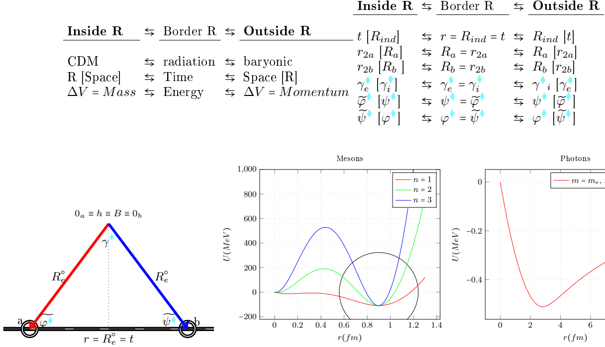
Figure 17. Photon: the photon is characterized by \gamma^\diamond = \pi/2 , L = 0 or \vartheta = 0 , E = h\nu , v = c and r = \overline{ah}^\diamond + \overline{bh}^\diamond = 2R_e^o
