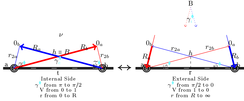
Figure 15. On the right the electromagnetic relation (i.e proton electron), which take place outside the radius R_{ind} where \gamma \rightarrow \pm\alpha/n and \gamma \rightarrow \gamma_i . On the left its inverse, the weak interaction (neutrinos), which takes place inside where \gamma \rightarrow \pi\pm\alpha/n and \gamma \rightarrow \gamma_e .
