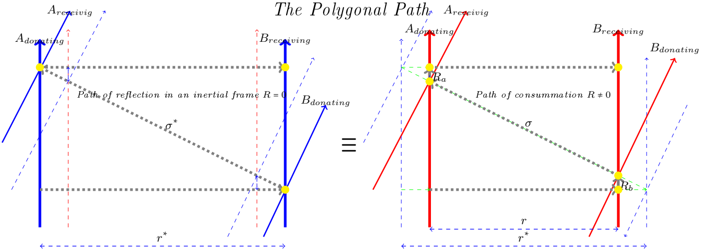
Figure 11. The Universal PATH: On the left the path of the reflection of light in an inertial frame. The planes of the Act of the two individuals intersect on the line of nodes and the thread equation is \sigma^* + r^* = \tau or V_i \sigma^* = \tau or \Delta\tau - \Delta\sigma = 0 . On the right, the real path of consummation, same time \tau and same angle \gamma . In this case, however, the path doesn't close on the line of nodes but on the radii R . Therefore the planes of act of the two conjoined individuals are separated by a distance R . Nevertheless the thread equation is R_b + \sigma + R_a + r = \tau or V_i \sigma + R_{tot} = \tau . Since the two spatial path must have the same length \tau , we have V_i \sigma + R_{tot} = V_i \sigma^* and therefore R_{tot} = V_i(\sigma^* - \sigma) . In particular, when \sigma = 0 we have d\tau = R_{tot} = V_i(\sigma^*) . Above all, from the intention scheme, V_i \sigma = t \cos \gamma^\diamond and therefore \tau = t \cos \gamma^\diamond - R_{tot} and \sigma = r + R_{tot} .
