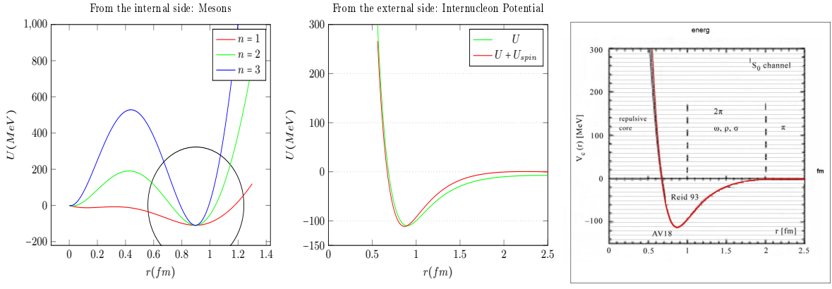
Figure 19. The internucleon potential: The plot of the eq. (35) when R^\circ = R_\epsilon^\circ = R_\epsilon^\circ/(2\pi) = 0.896978 fm and m_q = \alpha^{-1}m_\epsilon = \alpha^{-1}\pi m_\epsilon and \frac{L}{c} = \pi\alpha^{-1} .
