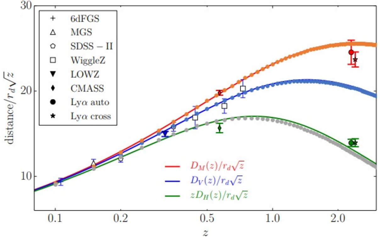
Figure 22. The BAO ‘‘Hubble diagram’’ (Aubourg \acute{E} . et al. 2014 [68] ) from a world collection of detections. Blue, red, and green points show BAO measurements of D_V/r_d , D_M/r_d , and zD_H/r_d , respectively, from the sources indicated in the legend. These can be compared to the correspondingly colored lines, which represents predictions of the fiducial Planck \Lambda CDM model (with m = 0.3183 , h = 0.6704 ) and the prediction of the Intention model (dotted line) when r_{s_{drag}} = 101.65/h Mpc. The scaling by \sqrt{z} is arbitrary, chosen to compress the dynamic range sufficiently to make error bars visible on the plot. Filled points represent BOSS data, which yield the most precise BAO measurements at z < 0.7 and the only measurements at z > 2 . For visual clarity, the Ly\alpha cross-correlation points have been shifted slightly in redshift; auto-correlation points are plotted at the correct effective redshift.
