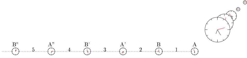
Figure 3. Recursive mirroring: two mirrors facing each other are reflected recursively. If there is a clock on each of them, from the reflected image present in every instant it is possible to reconstruct distances historically and therefore the velocities and accelerations over time, as far as the reflection allows.
