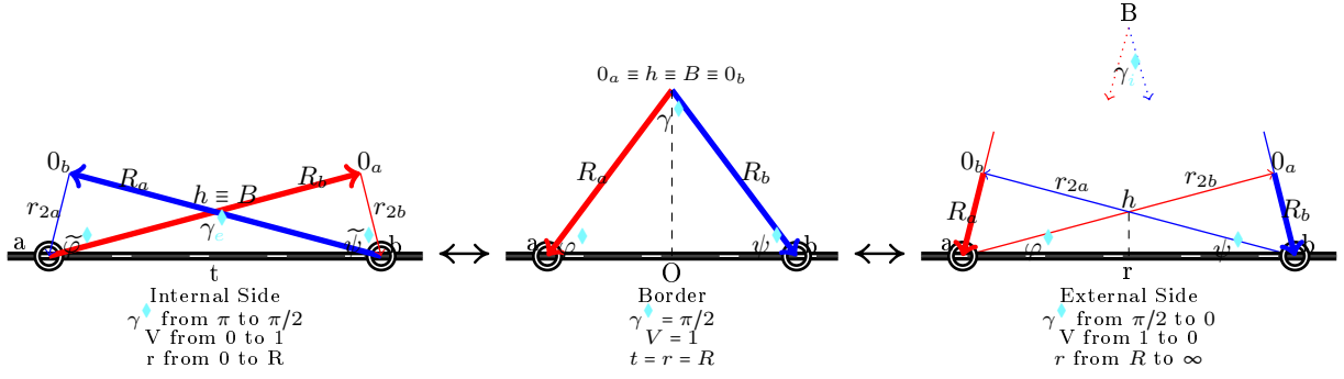
Figure 13. The intention schema when the interaction takes place respectively: On the internal side, on the border and on the external side.
