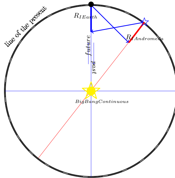
Figure 9. Intention Earth-Andromeda: The present, which comes from the Big Bang continuous as an approaching future, as soon as it surfaces, it submerge as past (antimatter) that move away to go towards the continuous Big Bang, and in this descent informs of itself the future (matter) that ascend in the opposite direction. In this way the past does not vanish but endures as it forms the future. This is the memory , which persists and is effective. The memory of the past that moves away from the present is the other face of the future that approaches, immersed in the potency. The further away it is, the more inexorably it is eroded by the waves of the potency and vanishes. Both faces are summarized in entropy which as a future that takes shape by approaching and emerging in the present, grows, as memory that fades away, decreases.
