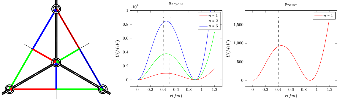
Figure 18. Baryon: the baryon is characterized by \gamma^\diamond = \pi/2 , \tilde{\varphi}^\diamond = \tilde{\psi}^\diamond = \pi/3 the plot of the universal equation (35). Strong Area repulsive force between three negative charge -1/3 : m = \pi 0.511 \text{ MeV} ; L = n \alpha^{-1} ; R^\circ = .896978 \text{ fm} .
