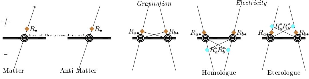
Figure 7. The sign of acceleration: The R_{\bullet} is advanced and therefore positive for matter. The mirror R^{\circ} , being reflected into the other, appears on the opposite side if the two conjugated individuals in the intention are homologue, on the same side elsewhere. Therefore, from the matter point of view, the acceleration is always attractive (time axes converge toward the future) for gravitation, while repulsive or attractive depending on the sign of the time axes for electromagnetism. All is reversed from the negative matter point of view
