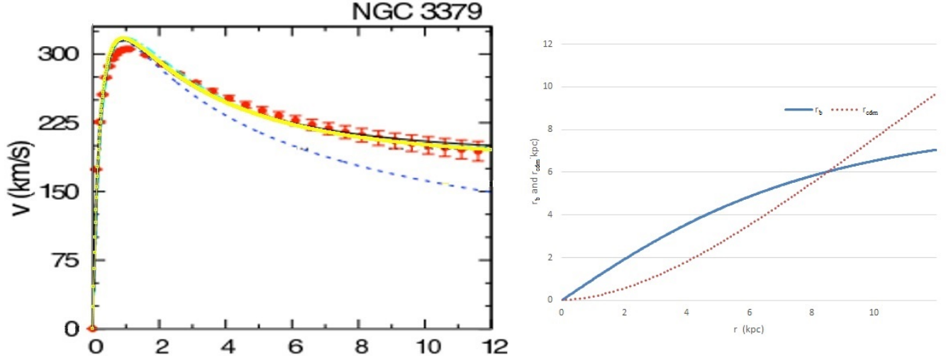
Figure 20. Rotation curve for the elliptical galaxy NGC 3379. The red points (with error bars) are the observations. The solid yellow line is the rotation curve determined by Intention Physics (eq. 54), the short dashed blue line is the Newtonian galaxy rotation curve. Both rotation curves are the best fit to a parametric mass distribution (independent of luminosity observations) a two parameter fit to the total galactic Mass, M = 6.99 \cdot 10^{10} M_\odot , and a core radius r_c = 0.45 kpc and \beta = 1 . On the right the trend of r_b and r_{cdm}
