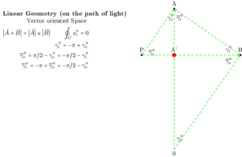
Figure 4. Linear spacetime of the act (on the path of instantaneous light): It is a Linear vector oriented space. The angles are \gamma_e between two vectors in concordant direction, vice versa \gamma_i , and they alternate each other.
