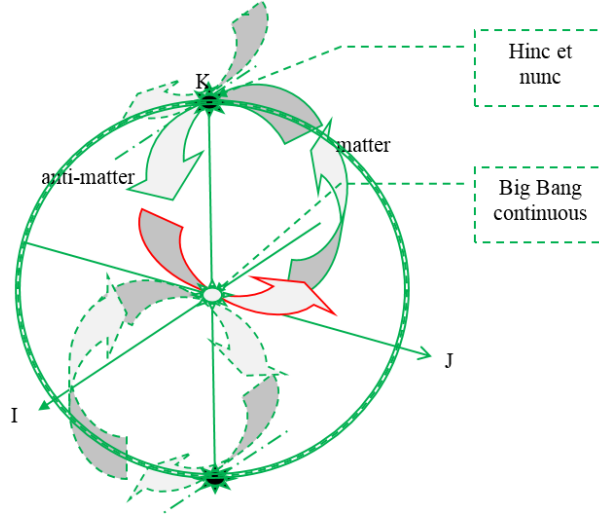
Figure 8. The Big Bang continuous: The radius and therefore the age of the universe is constant, and the Big Bang is not an event, but it is a part of a continuous process. The principle of reason claims that the present is based on the historical reconstruction of the past up to a starting point known as the Big Bang. The line of the present, on the opposite side, is the set of the points where matter coming from the Big Bang, after a period of potency lasted R_\omega years, emerges in act and reverses and begins its return journey in the potency as antimatter. The line of the present is the place where matter meets anti-matter and forms the baryonic matter (ordinary matter). The center of the line of the present, on the opposite side, is the point where all energy meets the anti-energy and gives rise to the Big Bang. Therefore, inside the universe, the total amount of energy is positive and equal to R_\omega , while all matter is exactly canceled out by antimatter.
