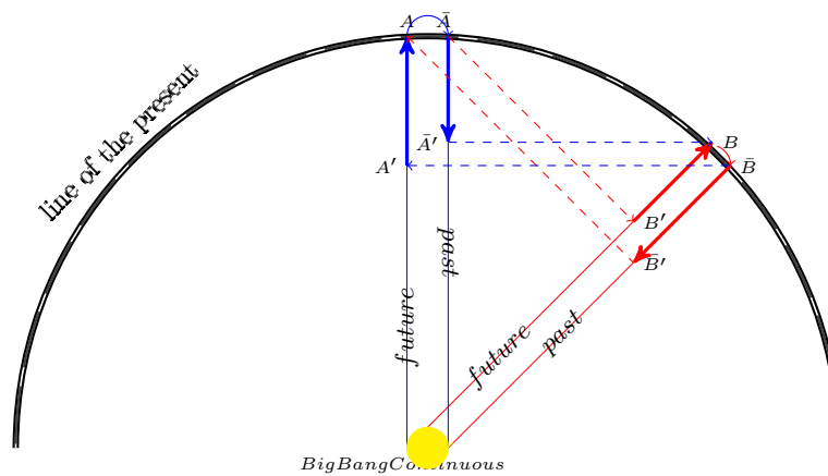
Figure 10. The path of universe intention: The cosmological intention between two individual A and B consists of two overlapping paths (in the figure they were separated to highlight each of them). The path of the present of A: 1) \bar{B}' \rightarrow A , 2) Ae^{i0} \rightarrow e^{i\pi}\bar{A} , 3) \bar{A} \rightarrow \bar{B}' , 4) \bar{B}' \rightarrow B , 5) Be^{i0} \rightarrow e^{i\pi}\bar{B} , 6) \bar{B} \rightarrow \bar{B}' . Analogously for the path of the present of B. Note that only on the line of the present and in the Big Bang the matter converts in antimatter. In the intention, the sending and receiving take place from the present of the individual who sends/receives, not to the present of the other individual, but to its embryonic potentiality (which approaches ascending from the Big Bang). This is why we, on the Earth, cannot communicate with distant alien civilizations. In fact we can not receive from (see) the present in which only they live and act, but from the embryonic potentiality. Equally we can not send to their present in act, but only to the embryonic potentiality of their future present.
