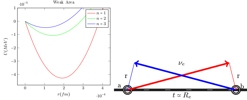
Figure 16. Neutrino: \pi m_e [-V + 1/2V^2 + 1/2(nL)^2V^2(1-V)^2] where R^\circ = .896978 and L = n\alpha^{-1} . There is one generation for each of the three angular momentum levels predicted by the weak interaction.
