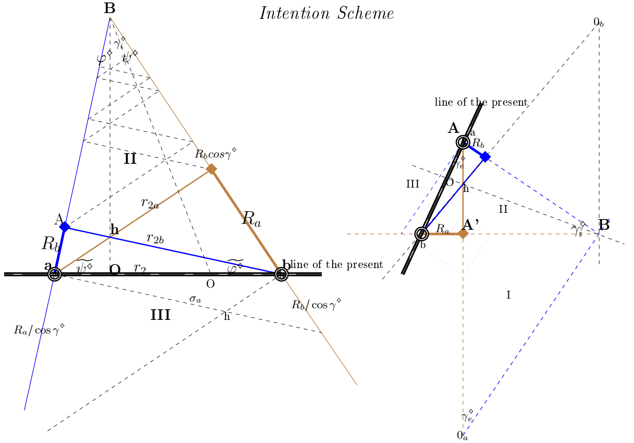
Figure 6. The whole relation is enfolded and unfolds from the Radii of the two conjoined individuals. The schema of intention is recursive since to every angle follows its opposite. Indeed the three quadrants represent time, space and potency and recursively follow one another. The Intention Schema, which emerges reflectively, represents all the possible knowledge on the relation and it is just a knowledge representation. Indeed, contrarily to the above schema, in every instant the receiving side of an individual face the parallel donating side of the other. Therefore, the intention schema, composed from the juxtaposing of homologue sides (donating-donating or receiving-receiving) of the two conjoined individuals, is only a construction for needs of knowledge representation. It is the begin of reflective knowledge which demands the determination of the angle \gamma of the relation given by the homologue side time of both individuals. In fig., two \overline{Oh} segments have been reported indicating the position of the center of gravity. Obviously the center of gravity is unique and coincident for both the gravitational and electrical relationship. In fact, where the largest gravitational Radius is also the smaller electric one and vice versa. In the diagram in the figure, therefore, an electrical relationship is represented, recognizable for having the (darker) center of gravity where the Radius is smaller.
