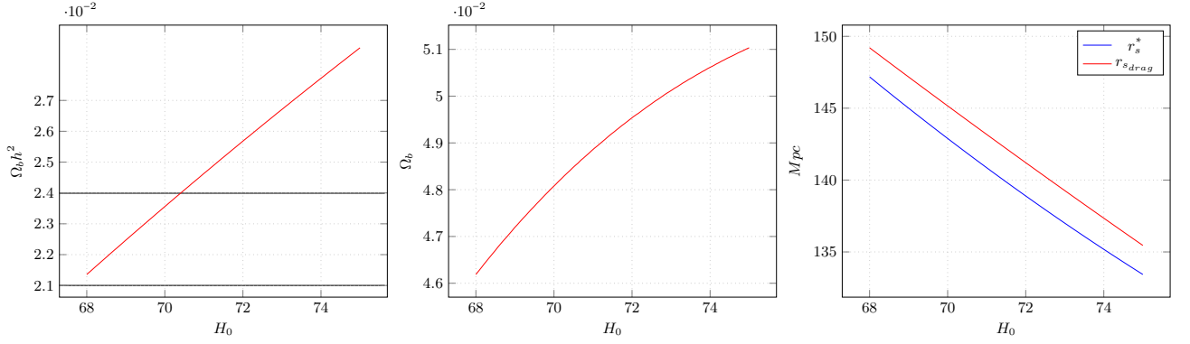
Figure 24. on the first and second panel the baryonic density as a function of the Hubble constant. The Big-Bang Nucleosynthesis predicts 0.021 \leq \Omega_b h^2 \leq 0.024 (95% confidence).
