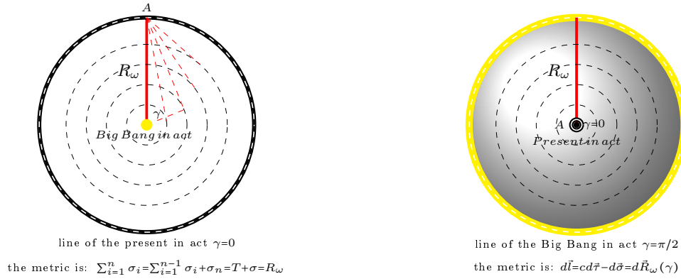
Figure 21. each individual on the line of the present has its own point of view on the universe Radius R_\omega . For each individual, every point in the universe Radius R_\omega represents a distance \sigma + T = R_\omega in the linear spacetime that turns in the isomorphic spherical surface of equidistant points in the three-dimensional quadratic space of potentiality. The space of potentiality, interposed between the big bang and the line of the present in progress, is three-dimensional and flat. In the present model all space-time is in potency, with the exception of the Big Bang and the line of the present in act, and every instant is all new and all present. Every instant the whole universe recurs unfolding itself from the Radius all interconnected.
