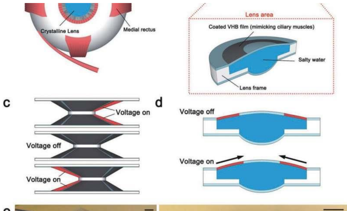
Illustration and photos of the soft robotic lens. Credit: Cai lab/Advanced Functional Materials
