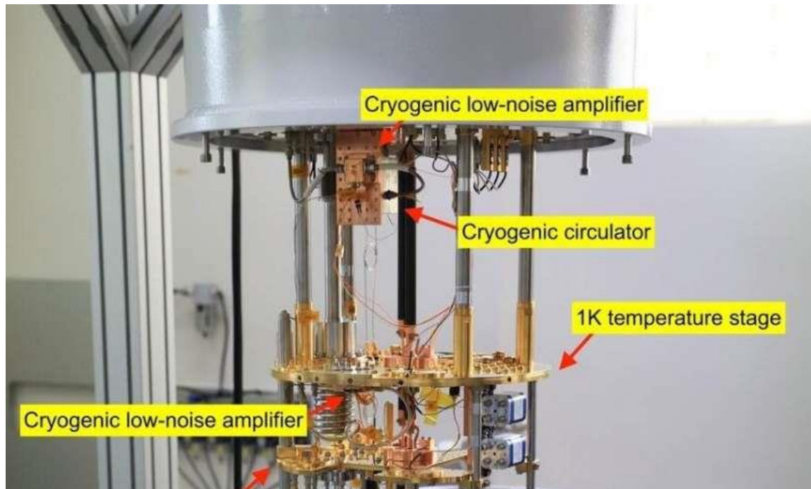
Figure 2. The CAPP-8TB experiment system. At the bottom, bore of the superconducting magnet (not shown in the photo) surrounds the resonant cavity, hanging on the lowest temperature stage. Various electronic components are placed at each temperature stage and further electronics are located outside the refrigerator. Credit: Institute for Basic Science
