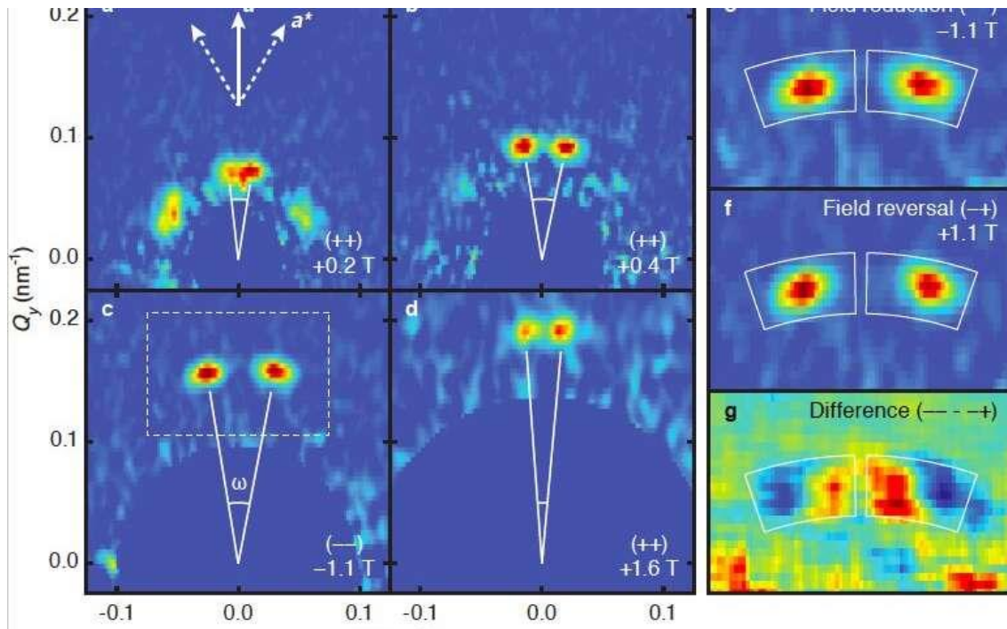
Vortex-lattice (VL) diffraction patterns. Credit: Avers et al
