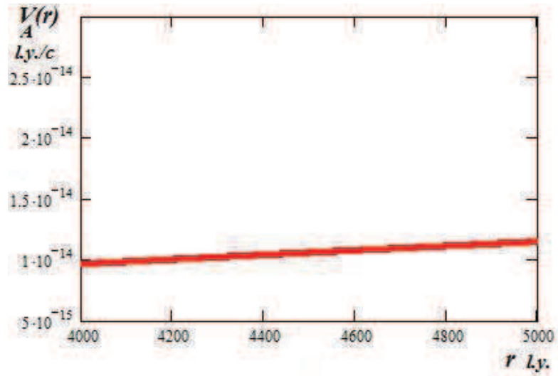
Figure 13: Dependence of V_A(r) on r with x_A = 25 \times 10^3 \text{ l.y.}
