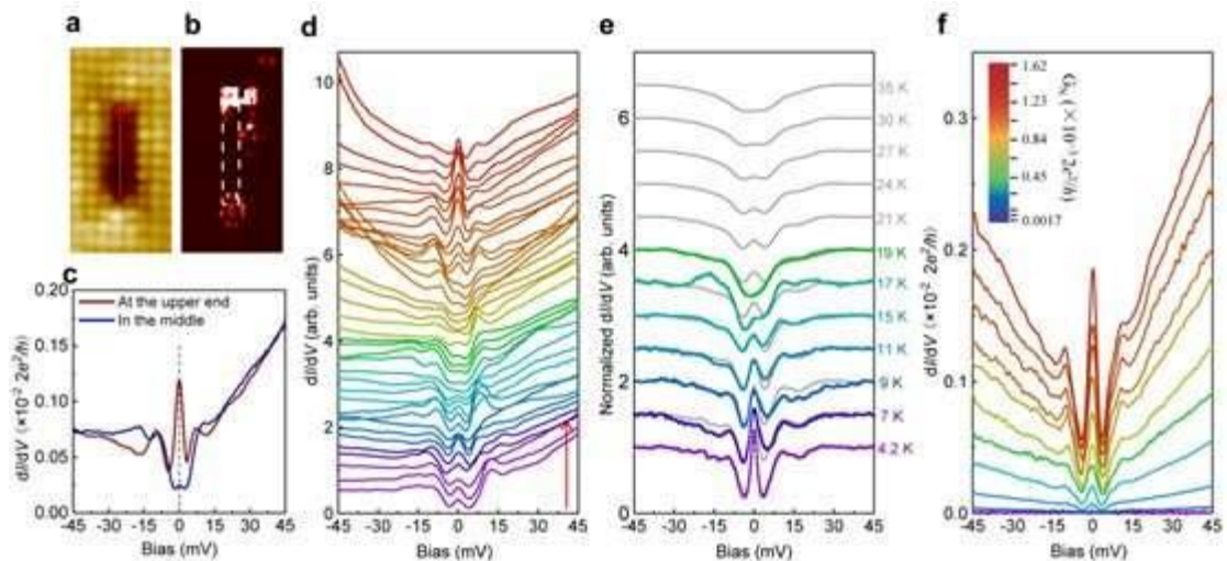
Figure 2. ZEBs at the ends of a short atomic line defect (about 8 Te/Se atoms in length). a, An STM topographic image of the short 1D atomic line defect. b, Spatial zero-energy mapping. c, Tunneling spectra measured at the upper end and in the middle of the atomic line defect. d, Tunneling spectra taken along the red arrow direction in a. e, The temperature evolution of the ZEBs at the top end of the line defect. The coloured curves are normalized tunnelling spectra and the grey curves are the 4.2-K spectra convoluted by the Fermi–Dirac distribution function at higher temperatures. f, The tunnelling barrier dependence of the ZEBs at the top end of the line defect. Credit: Peking University
