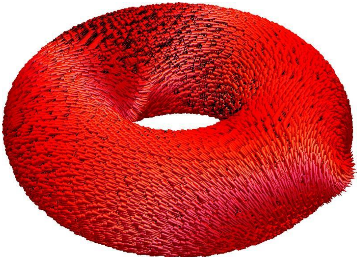
Doughnut-shaped nanomagnets induce new magnetization states
