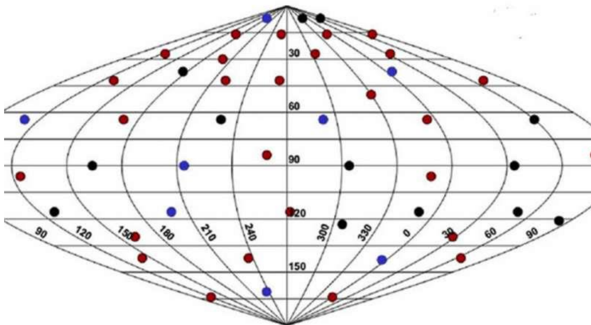
Distribution of RT-NADs detectors on the NIF target chamber. The red dots indicate locations where holes were drilled to insert the detectors. Credit: Lawrence Livermore National Laboratory
