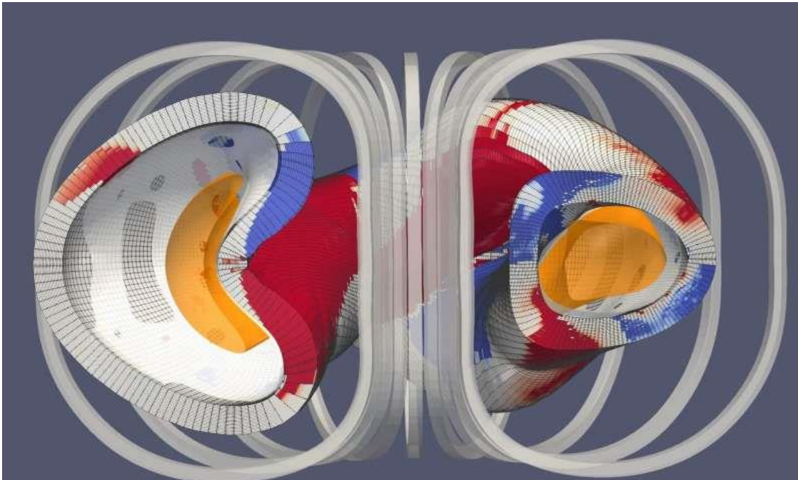
Schematic image of permanent magnet stellarator with plasma in yellow. Red and blue indicate permanent magnets with simplified coils surrounding the vessel. Credit: Coaxing Zhu.
