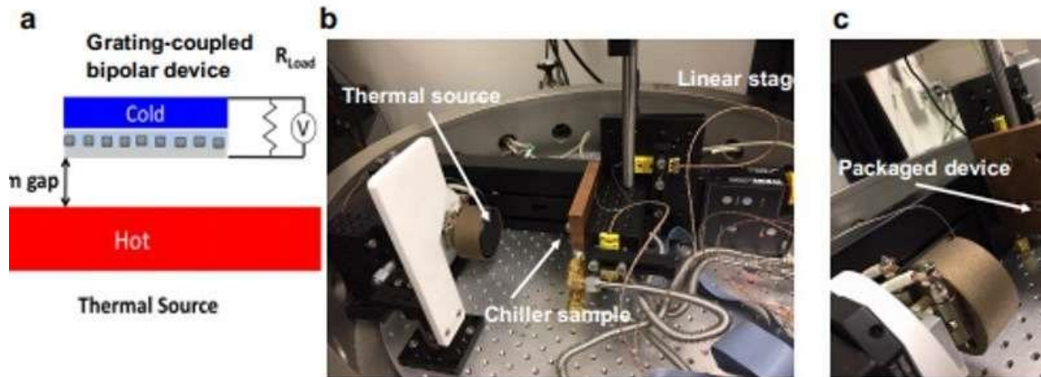
Vacuum thermal photovoltaic measurement system (a) Schematic device configuration for thermal to electrical power conversion. R_{Load} is a variable load resistance outside of vacuum. (b) Circular heater coated with blackbody high emissivity paint used for thermal source. Sample is on chilled copper block mounted on a linear stage for position control. (c) Packaged sample is flush mounted and electrically contacted from the backside with thermocouples mounted to front of sample and backside of sample package for temperature monitoring. Credit: Science Advances, doi: 10.1126/science.aba2089
