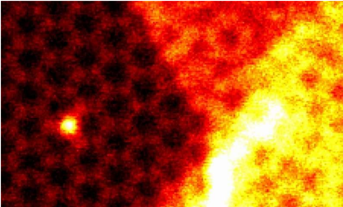
An image taken from an electron microscope showing the single atom of silicon in the graphene crystal. It is brightly coloured and to the left hand side of the image. Credit: Q. Ramasse, SuperSTEM
