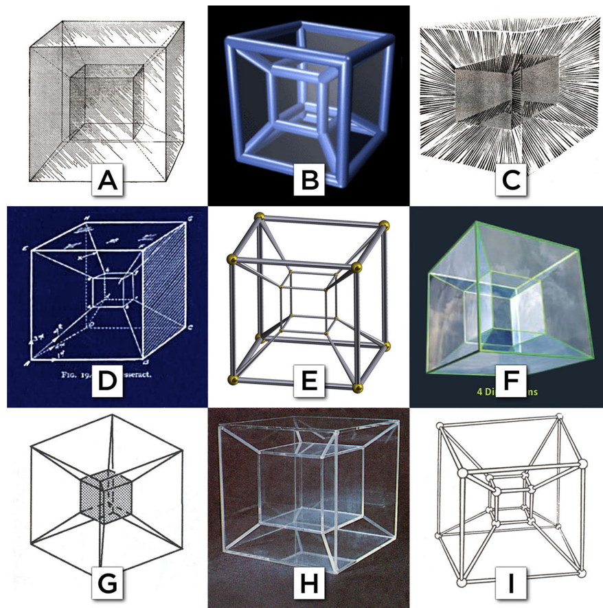
Fig. 10. – Hypercube (Tesseract) Gallery: A) Claude Bragdon; B) Wikipedia; C) Martin Gardner; D) Alexander Horne; E) Victor Schlegel; F) Jan Ambjørn, et al; G) Clifford Pickover; H) Carl Sagan; I) Rudy Rucker. The geometer Thomas Banchoff has described a tesseract as a “head-on view” or a “central projection” of a four-dimensional cube. Motivated entirely by geometrical, as opposed to physical considerations, these images are all supposed to represent an “extra” spatial dimension, which is just as static as the first three. I.e., there is no explicit, or even implicit relationship to matter, time, or gravity. Whereas in the Rotonians’ Space Generation Model, the relationships are such that no space at all would exist were it not that matter is perpetually generating space by moving, with the unfolding of time, into (or outfrom) the fourth spatial dimension.
