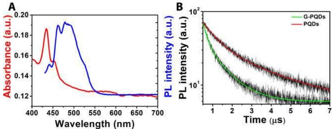
UV-vis and PL spectra. (A) Ultraviolet-visible (UV-vis) absorption (red) and PL spectra (blue) of the G-PQD superstructure film. (B) PL decay profiles of PQD (red) and G-PQD films (green). Credit: Science Advances, doi: 10.1126/sciadv.aay5225
