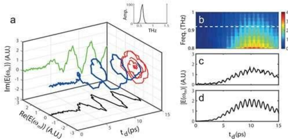
Figure 2. The complex amplitude of light at the converted frequency with the variation of a spatiotemporal boundary. Credit: The Korea Advanced Institute of Science and Technology (KAIST)
