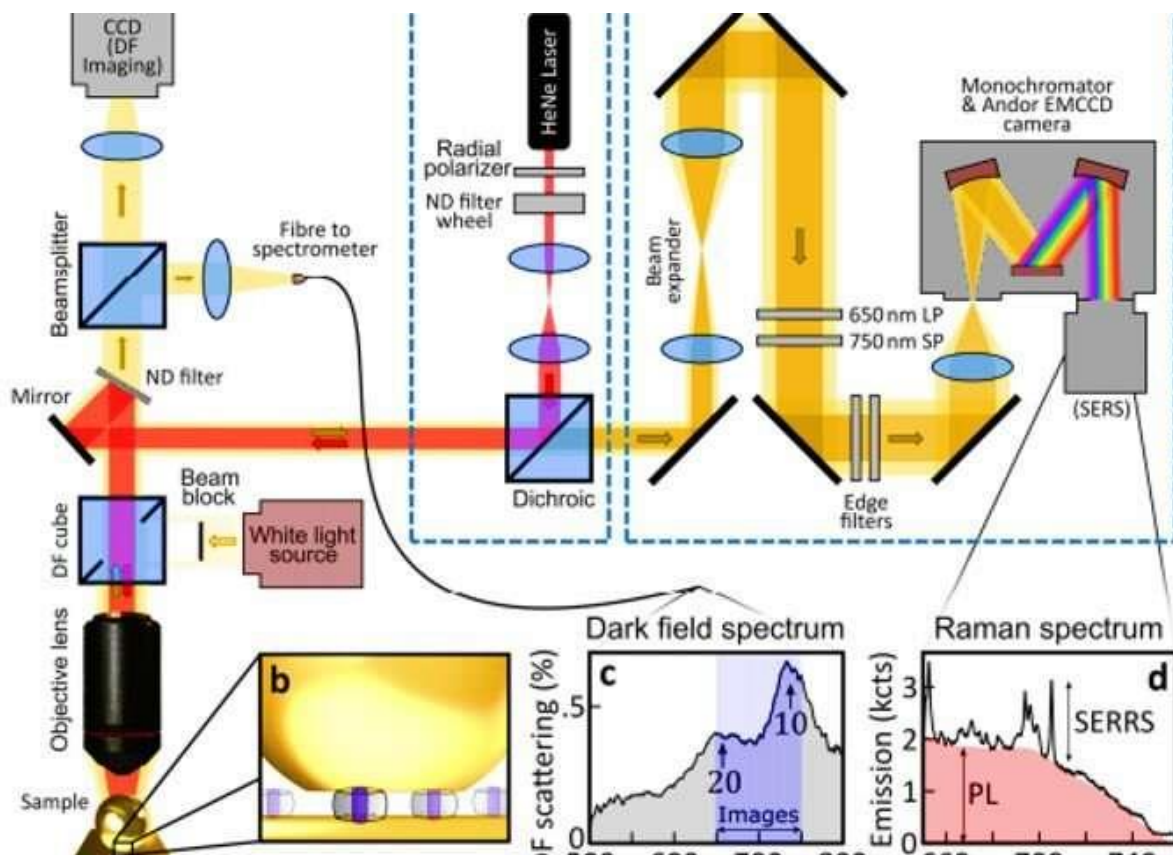
Experimental setup. a, Schematic of both imaging and spectroscopy. Left side shows imaging system used for alignment, automatic sample scanning, and collection of DF spectra. Boxed section 'Raman laser' shows radially-polarized 633 nm excitation laser used in collection of emission images and spectra. Boxed section 'Raman spatio-spectral detection' shows separation of emission from excitation, magnification stages, imaging, and collection of emission spectra. b, Schematic of typical NPoM, with a flat facet and a CB[7] spacer layer (not to scale). c, Dark field scattering spectrum of a typical NPoM with a ring-shaped emission and d, emission spectrum. Credit: PNAS, doi: https://doi.org/10.1073/pnas.1914713117
