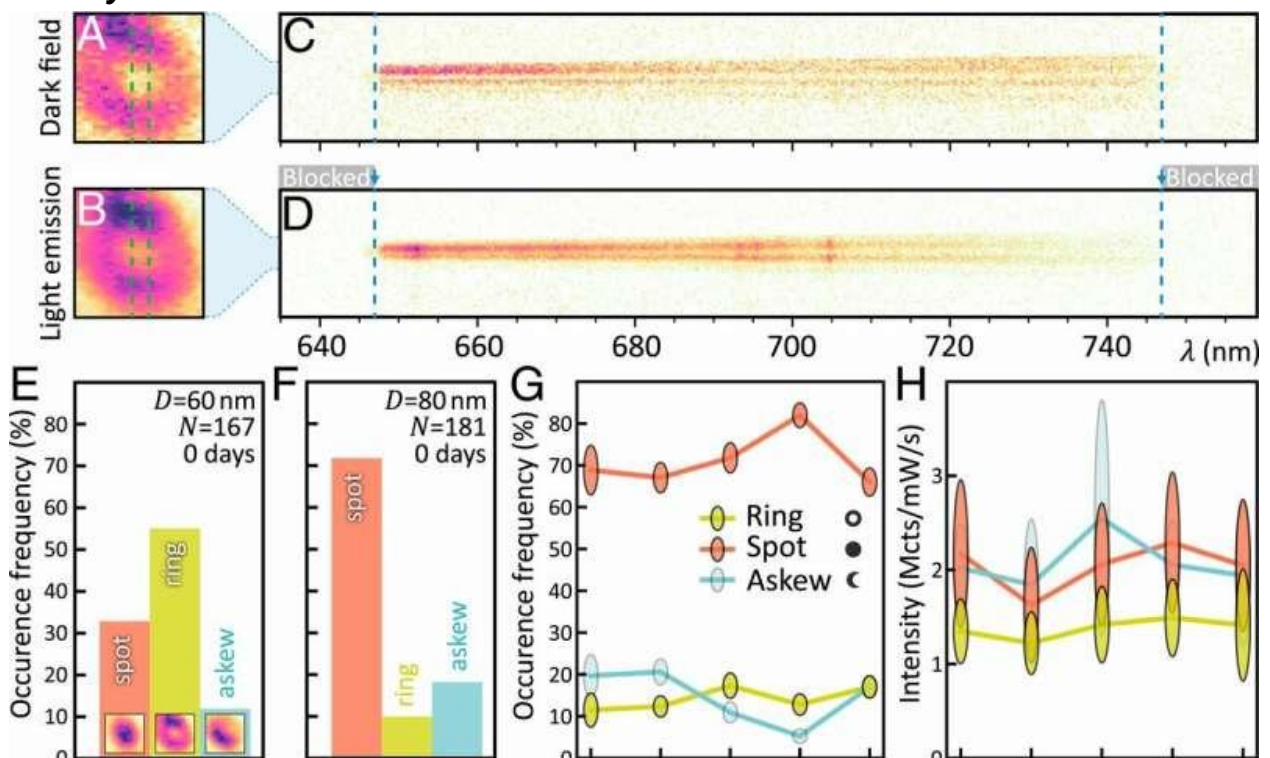
Real-space scattering and emission images from single NPOMs. (A and B) Spectrally integrated (647–747 nm) images of white-light dark-field scattering and light emission (in “ring” state). (C and D) Spectrally resolved emission through a vertical cross-section formed by the entrance slit (dashed lines in A and B) showing ring profile for both broadband PL and sharp SERS lines. (E–G) Relative occurrence of each shape (E, Insets) for D = 60-nm (E) and 80-nm (F and G) NPs. (H) Integrated emission intensity of 80-nm NPs, as sample ages after initial preparation. Vertical ellipses give SEs of fractions (G) and intensities (H) from N(t) NPs. Credit: PNAS, doi: https://doi.org/10.1073/pnas.1914713117
