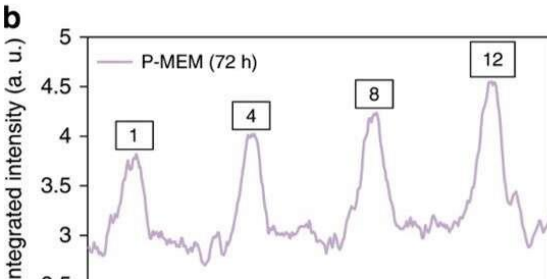
Exploring the limits of the P-MEM property. (a) Digital picture of the sample during irradiation of the phosphor with IR radiation 72 h after mechanical stimulation, consisting of a sequence of drags. (b) Integrated intensity profile derived from a, showing the P-MEM intensities corresponding to 1, 4, 8 and 12 drags. Credit: Light: Science & Applications, doi: 10.1038/s41377-019-0235-x
