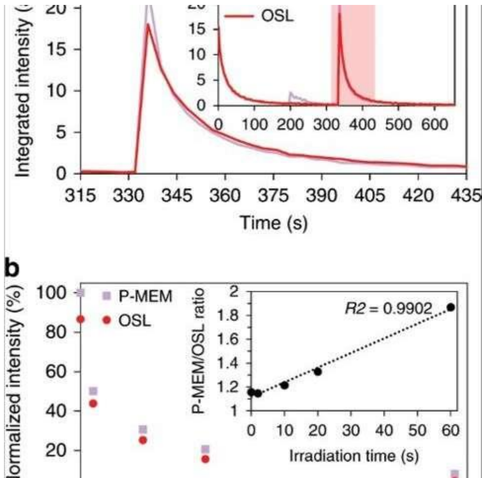
MEM signal visibility. (a) Temporal behaviour of the P-MEM signal. The inset shows the complete duration of the experiment with periods of afterglow (first ~180 s), mechanical stimulation (~180–250 s) and IR irradiation (~330–600 s). The highlighted area is shown in detail in the main figure. (b) Effect of pre-irradiation on the OSL and P-MEM intensity, leading to an increase in contrast between both signals, as shown in the inset. Credit: Light: Science & Applications, doi: 10.1038/s41377-019-0235-x
