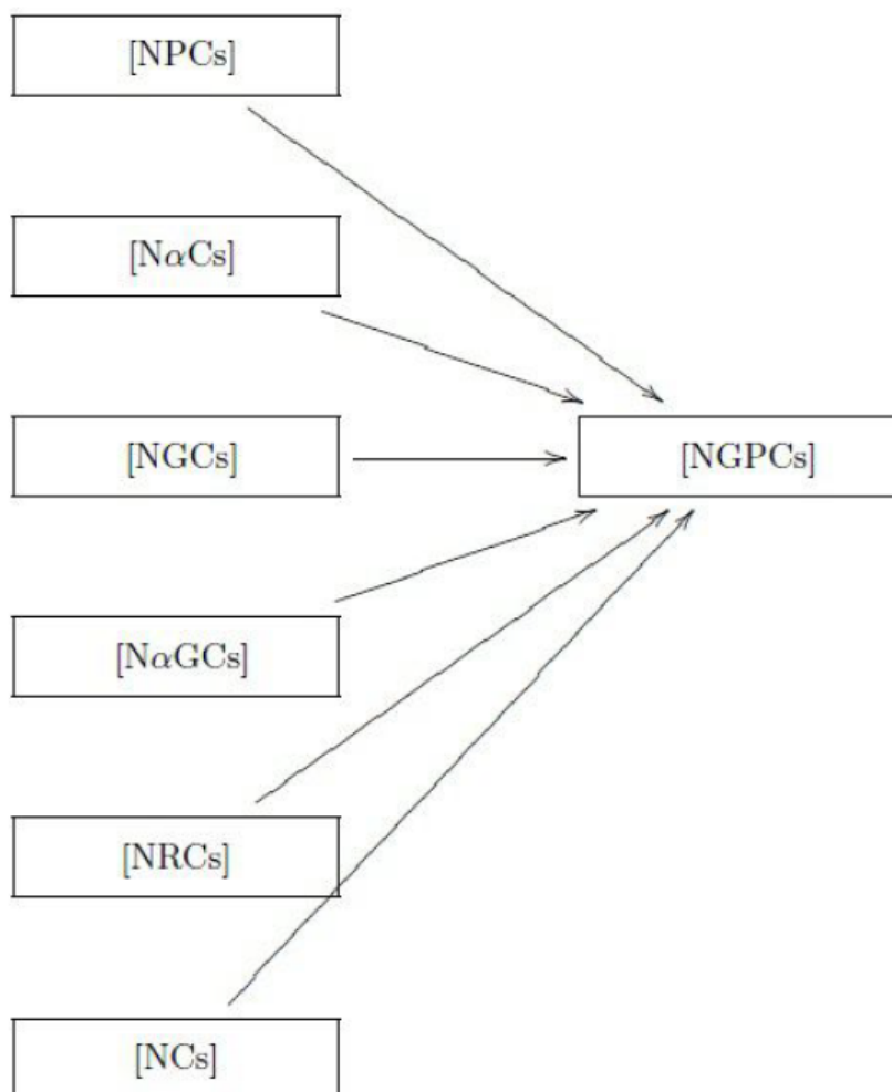
Figure 1. Relations between GNPC and other existed sets.
