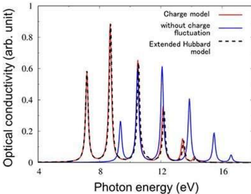
Comparison of optical conductivity spectra between the charge model and the extended Hubbard model. Optical conductivity spectra for a system consisting of 14 atoms are shown. The spectrum calculated from the charge model (red solid line) quantitatively coincides with that calculated from the extended Hubbard model (black broken), while that calculated without charge fluctuation (blue solid) shifts about 2 eV (electron volt). Credit: 2009 The American Physical Society
