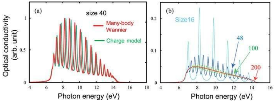
Optical conductivity spectra calculated by using many-body Wannier functions. (a) Comparison of the charge model and the method of the many-body Wannier functions. The method of the many-body Wannier functions well reproduces the optical conductivity spectrum calculated from the charge model for a system consisting of 40 atoms. (b) System size dependence of the spectra calculated by using the many-body Wannier functions. The spectral distribution becomes broad as the system size increases until the size reaches about 200. Credit: 2009 The American Physical Society
