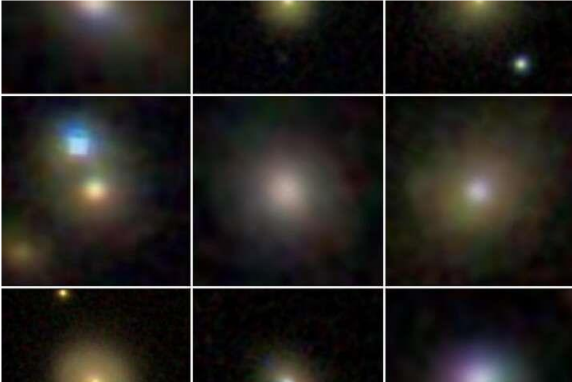
Dwarf galaxies hosting active galactic nuclei that have spatially extended outflows. Credit: SDSS.
