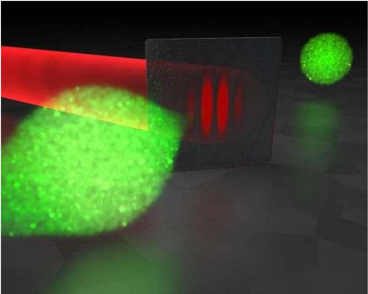
Electrons (green) reshape into tilted pulses by interference with a beam of laser-generated terahertz radiation (red) Credit: Copyright: Baum
