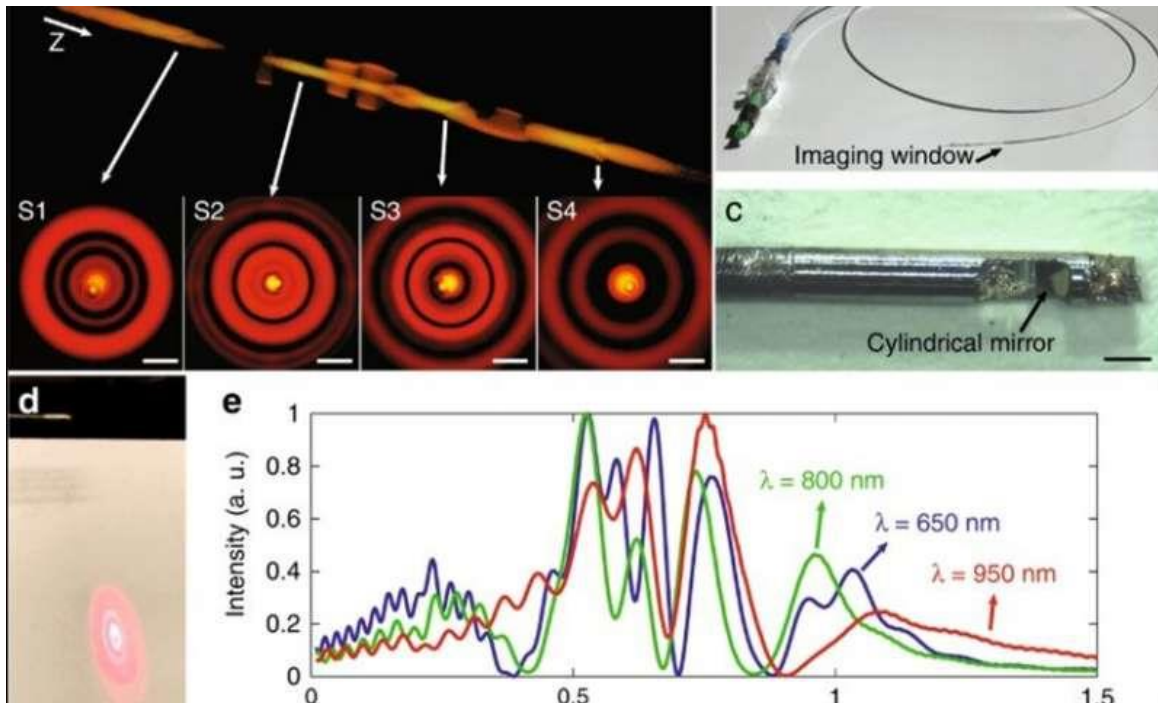
(a) Simulation of the aberrated beam field intensity when scatterers are positioned at the center of the beam path. Four scatterers were modelled, denoted as S1–S4. The scatterers had a diameter of 2 \mu\text{m} and a refractive index of 1.5. 3D rendering of the beam field and the transverse intensity distributions show that the aberration introduced by an individual scatterer is confined within each mode. Z indicates the beam propagation direction. Scale bar: 10 \mu\text{m} . (b) Photograph of the completed 2.6-F rapid guidewire exchange coronary catheter. (c) A photograph of the distal end of the catheter, taken using a microscope. The fibre probe had a diameter of 500 \mu\text{m} and a rigid length of less than 4 mm. Scale bar: 500 \mu\text{m} . (d) Photograph of the ring pattern of the light transmitted through the catheter's fibre probe optics, corresponding to multiple propagation modes. The screen was positioned at a small angle with respect to the beam propagation direction, showing that the cylindrical mirror directs the beam at an \sim 8^\circ angle normal to the sheath to reduce specular reflection. (e) Simulation of the normalized on-axis field intensity distribution with respect to depth for the center wavelength and the two ends of the spectra, showing that the chromatic focal shift effect mitigated the field intensity discontinuity. Credit: Light: Science & Applications, doi: 10.1038/s41377-019-0211-5
