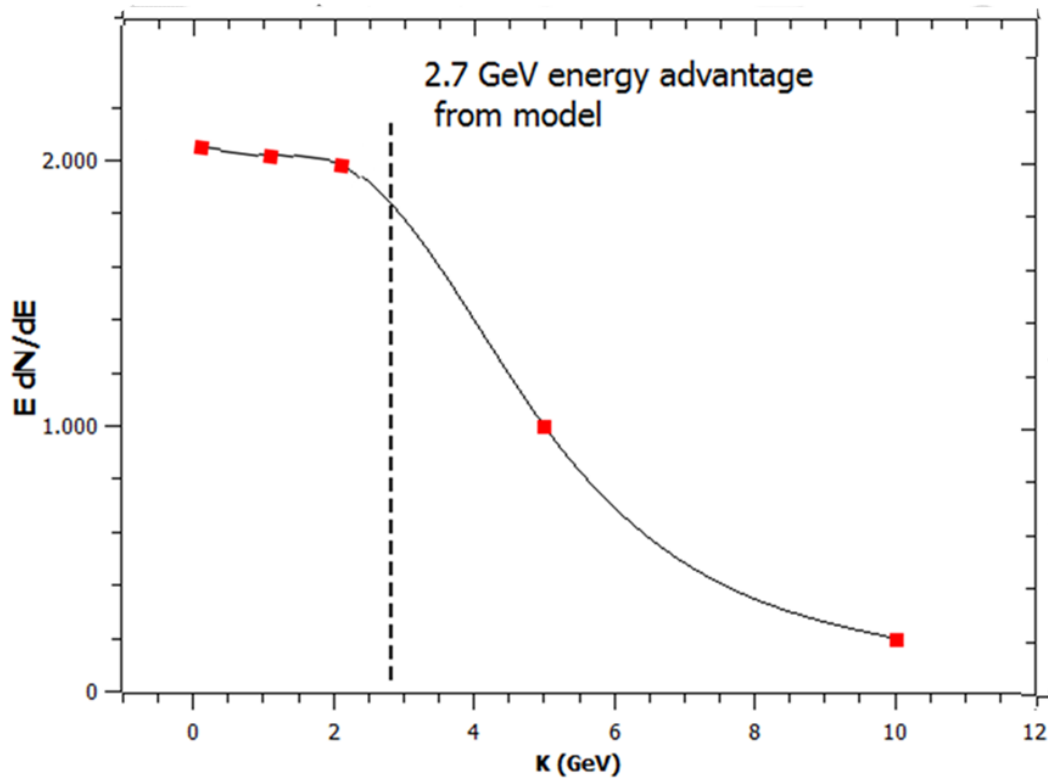
Figure 1: Reproduction of the upper left part of the double-log plots in Figure 1.1 of ref.[3] ( linearized scales are adopted here). The number flux of protons in 10^3 (\text{m}^2 \cdot \text{sr} \cdot \text{s})^{-1} units is plotted against the protons kinetic energy in GeV. The vertical line is placed at the value of K that corresponds to total loss of the vortex energy advantage compared to the vacuum parent state( see [1]). Integration shows that 80% of N concentrates below 3 GeV energies. The solid line is a guide.
