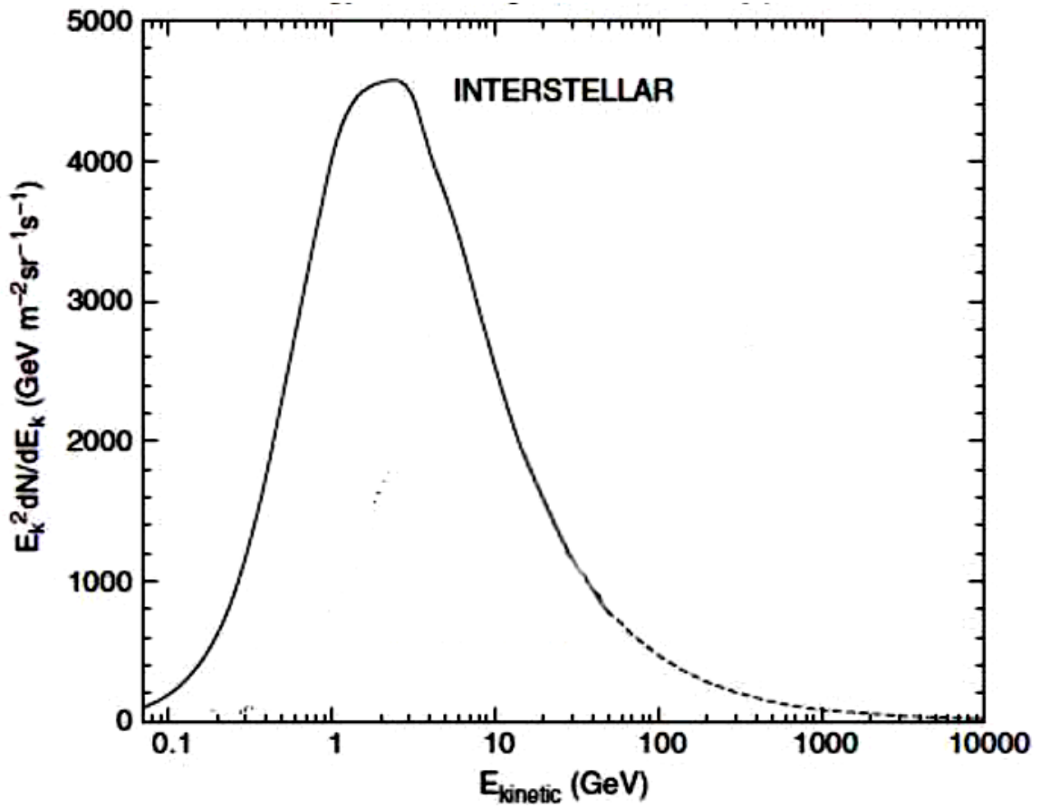
Figure 2: Corrected energy flux distribution of interstellar protons in cosmic rays, which average is about K= 2.7 GeV[3].
