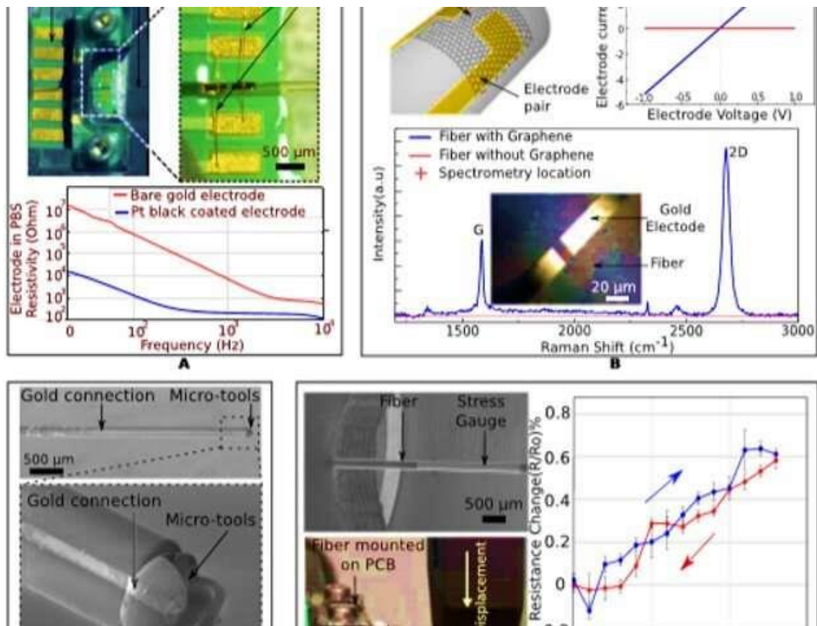
Example applications of microrobot-assisted wet transfer for fiber functionalization. (A) Top: Interface between fiber-supported electrodes and a dedicated PCB. Bottom: Impedance characterization of a two-electrode device with and without electrodeposition of Pt black. (B) Fiber-based 2D graphene devices. Sequential wet transfers were made to successively pattern the Au track and then the graphene film. The presence of graphene was assessed with Raman spectrometry and a plasma destructive test. (C) SEM picture of a functionalized microtool 3D printed to the tip of a fiber. The Au track was aligned and transferred onto the 3D structure with good conformity. (D) Fiber-based strain gauge designed for measuring fiber deformation based on its resistivity change. SEM picture of the device, picture of the experience, and resulting signal. Credit: Science Robotics, doi: 10.1126/scirobotics.aax8336
