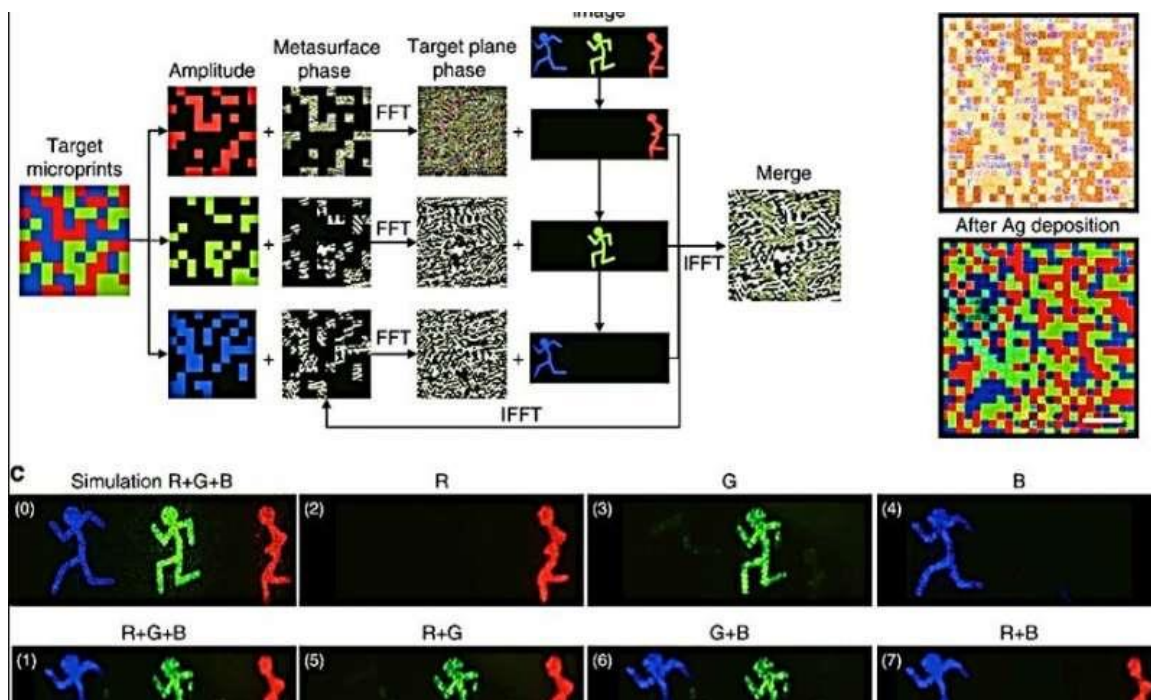
Concept demonstration of the 3D-integrated metasurfaces. (a) The flowchart of the modified Gerchberg–Saxton (GS) algorithm to generate the hologram phase. FFT is the fast Fourier transform, and IFFT is the inverse fast Fourier transform. (b) Transmission images of a random trichromatic colour microprint with 24 \times 24 pixels captured by an optical microscope: before (top) and after (bottom) the deposition of the top silver layer. The scale bar is 50 \mu\text{m} . (c) The far-field hologram images of “running man” captured by a digital camera on a screen: (0) the simulation result of R + G + B channels; (1)–(7) seven channels achieved by combining the RGB in the experiments. Credit: Light: Science & Applications, doi: 10.1038/s41377-019-0198-y
