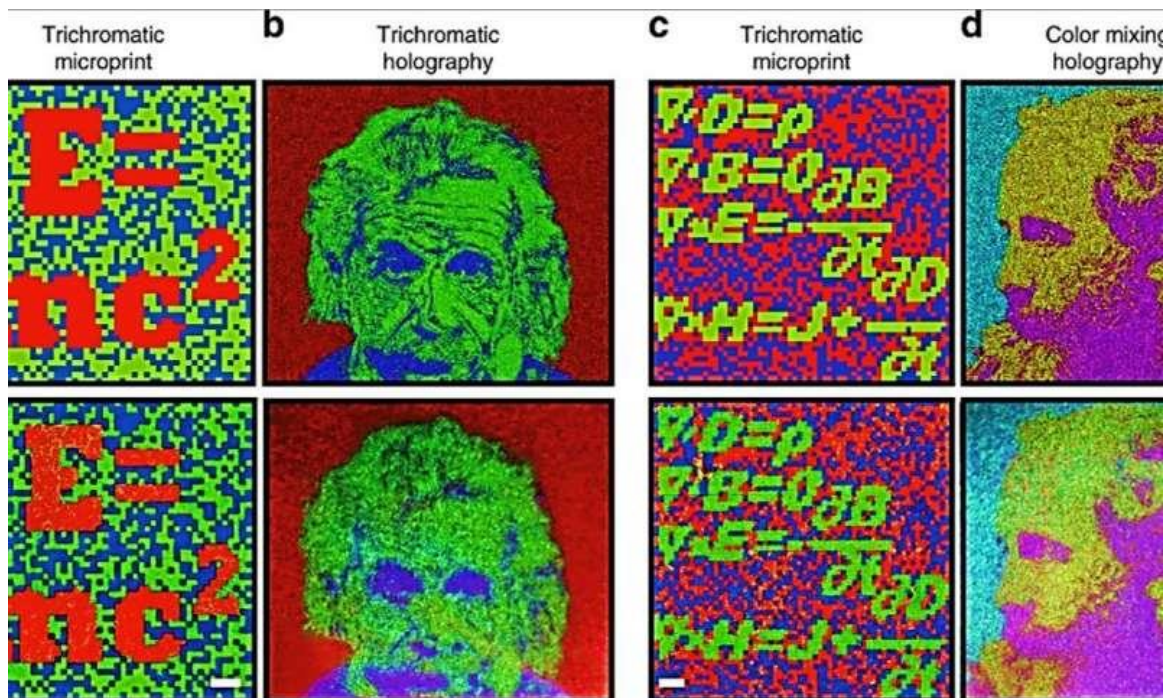
Two 3D-integrated metasurfaces for optical encryption: (top row) simulations and (bottom row) experiments. (a) Mass-energy equation in the trichromatic microprint with 50 \times 50 pixels. (b) Trichromatic portrait of Albert Einstein in a hologram image. (c) Maxwell equations in the trichromatic microprint with 60 \times 60 pixels. (d) Mixed color portrait of Jams Clerk Maxwell in the hologram image, demonstrating the combination capability of RGB channels to obtain yellow, purple, and cyan colors. The scale bars in (a) and (c) are 50 \mu\text{m} . Credit: Light: Science & Applications, doi: 10.1038/s41377-019-0198-y
