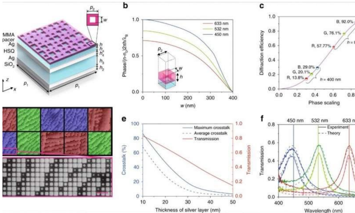
Design and fabrication of 3D-integrated metasurfaces. (a) Schematic of a unit cell of the 3D-integrated metasurfaces. (b) The phase change normalized based on the B channel with varied sizes of nanoholes. (c) The diffraction efficiency with different phase scaling and B, G, and R efficiency of PMMA with a refractive index of 1.48 in the visible light range at 400 nm (29.0%, 20.1%, and 13.8%) and 800 nm (92.0%, 76.1%, and 57.8%, respectively) height. (d) False-color SEM image of the device with a color filter microarray (unit size: 10 \mu\text{m} ) and hologram metasurface (structure period: 400 nm). Different colors represent the separated color filters in the device. Scale bar: 1 \mu\text{m} . (e) Effect of silver film thickness (the thickness of the two silver films is equal) on maximum crosstalk, average crosstalk and transmission efficiency. Increasing the silver film thickness can suppress crosstalk, but it also reduces transmission efficiency. (f) Theoretical and experimental transmission spectra for R (633 nm), G (532 nm), and B (450 nm) channels of 26-nm-thick silver layer color filters (dark-color serial line) and 31-nm-thick silver layer color filters (light-color serial line). Credit: Light: Science & Applications, doi: 10.1038/s41377-019-0198-y
