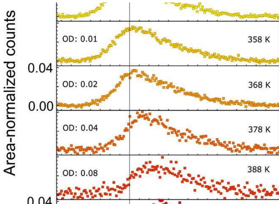
Area-normalized temporal photon shapes. Area-normalized temporal shapes of frequency-converted photons that have passed through a warm ^{87}\text{Rb} vapor cell. The ^{87}\text{Rb} vapor cell temperature is set to the values indicated. The optical density (OD) of the warm vapor is stated for each temperature, at a frequency \omega_0 , and using the same atomic density, N . Credit: Science Advances, doi: 10.1126/sciadv.aav4651
