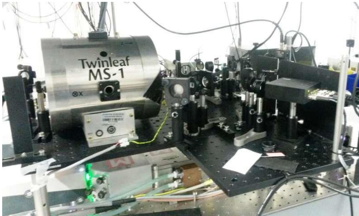
Experimental setup for atomic spectroscopy using cesium atom vapor. Credit: Dionysis Antypas
