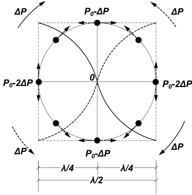
Figure 3. Schematically is designed the harmonic fluctuation of motion arrow \Delta P = (P_0 - \Delta P) - (P_0 - 2\Delta P) of the particle spin
