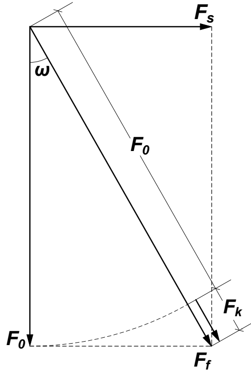
Figure 4. F_k = F_f - F_0 is the kinetic force of a particle, F_f its final force, F_0 its gravity force, u_a = F_s/F_f = \sin\omega its timeless speed 15 and F_f^2 = F_0^2 + F_s^2 is the Pythagorean 16 relationship
