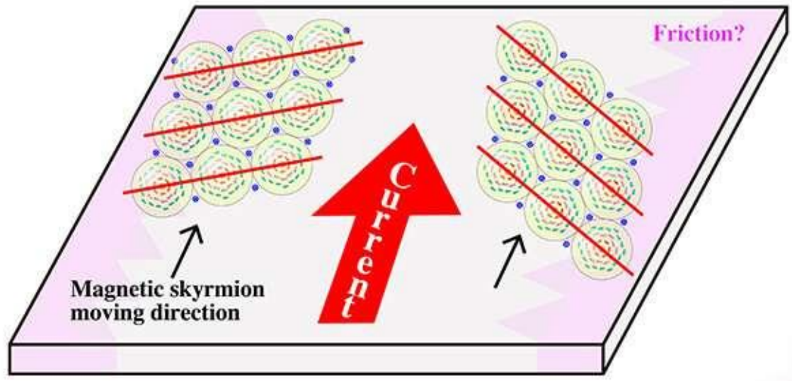
Researchers speculate that the magnetic skyrmion lattice moves the same direction with the applied electric current direction. Near the sample edge, the plastic deformation of the magnetic-skyrmion lattice takes place, resulting in the counter-rotating behavior of the magnetic skyrmion reflections. Credit: D. Okuyama, Tohoku University
