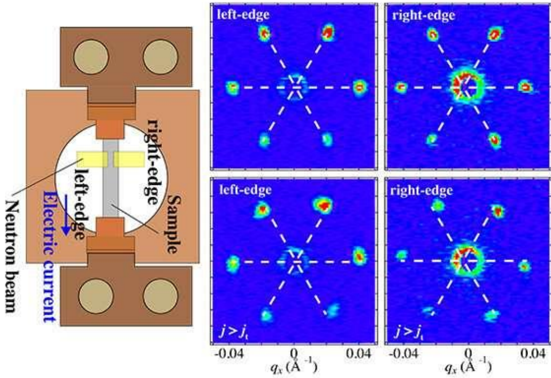
Magnetic reflections from the skyrmion lattice in MnSi. Credit: D. Okuyama, Tohoku University
