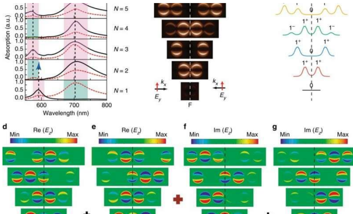
Plasmonic encoding in gold nanodisk chains. a Calculated absorption spectra of gold nanodisk chains consisting of different numbers of nanodisks illuminated by the s-polarized in-plane plan wave coming from right side (dashed line) or both ... more
