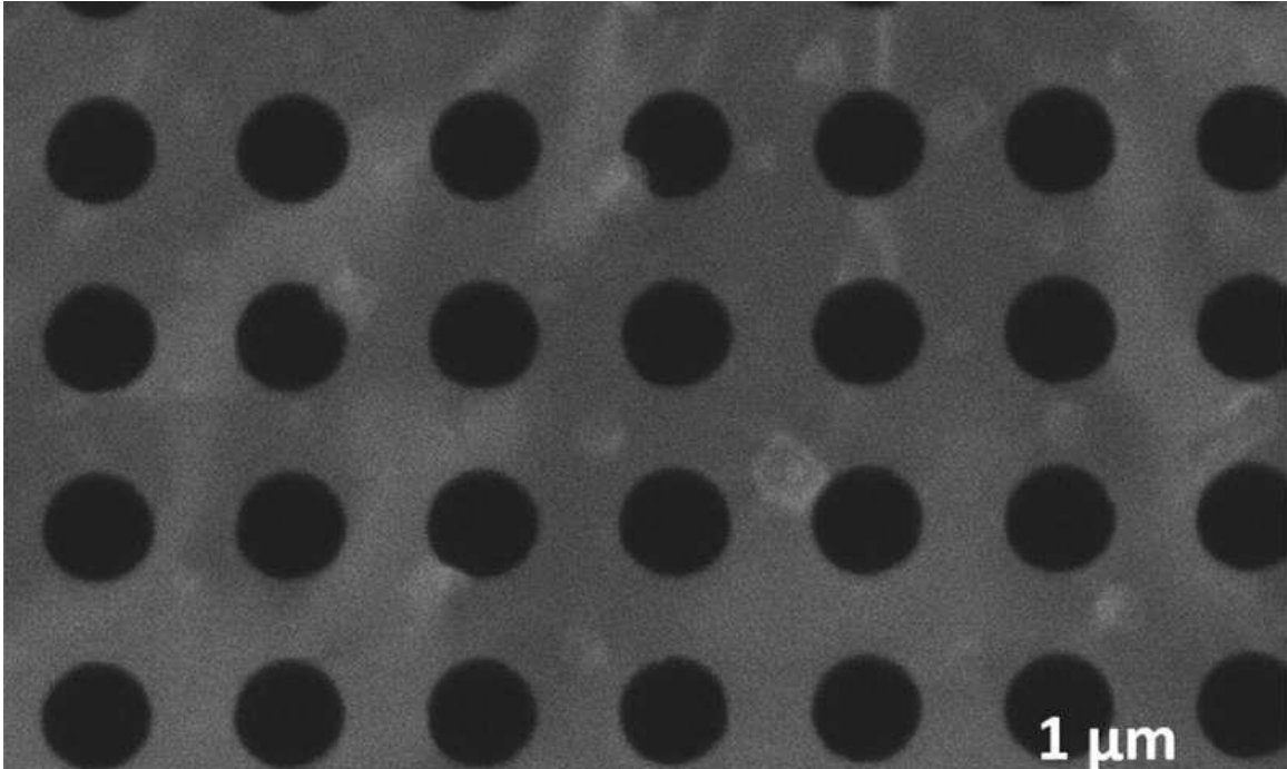
SEM image of the waveguide structure: a suspended tungsten disulfide monolayer patterned with nanosized holes. Credit: Cubukcu lab
