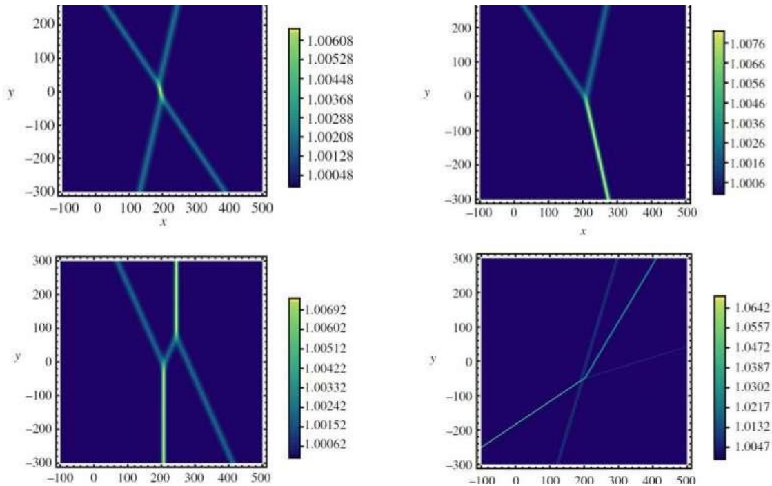
Simulation results showing different patterns emerging in optical soliton interactions. Credit: Horikis and Frantzeskakis. ©2019 The Royal Society
