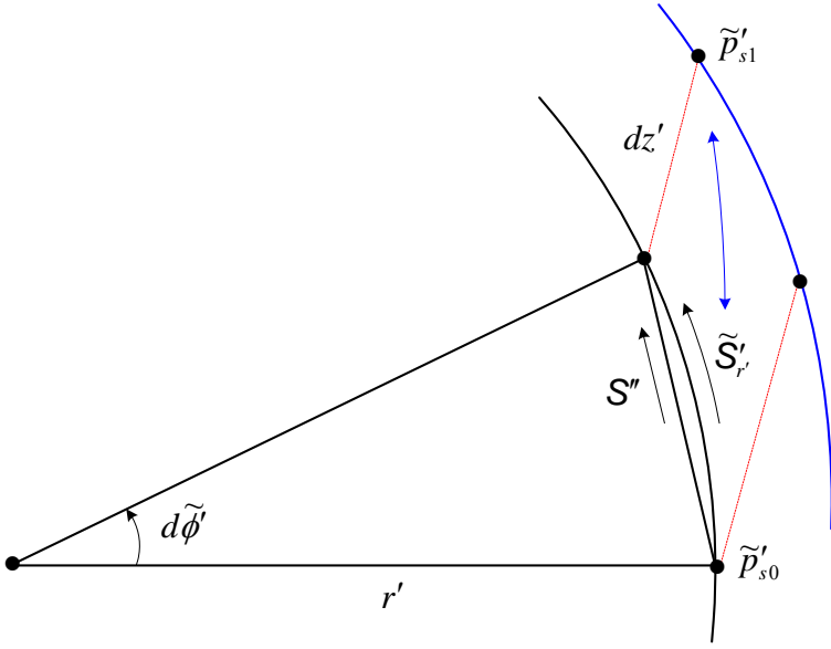
Fig. 3. World systems \tilde{S}'_r and S'' .
