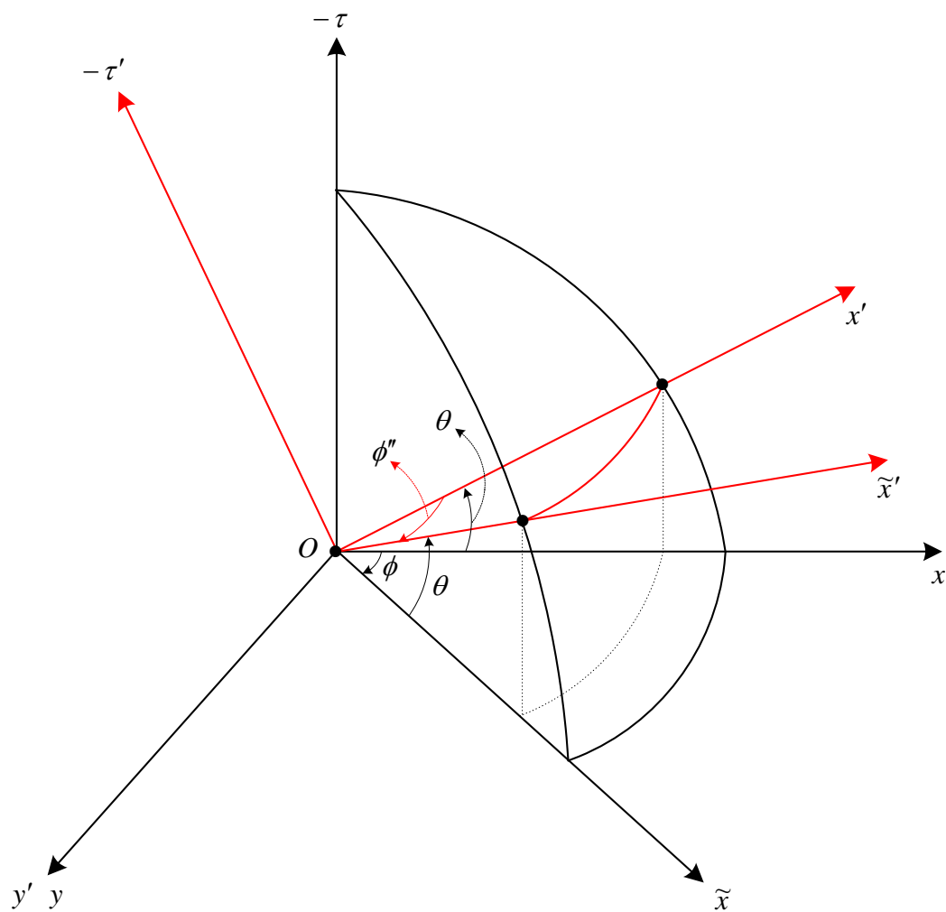
Fig. 1. Unprimed coordinate systems S and \tilde{S} and primed ones S' and \tilde{S}' corresponding to S and \tilde{S} , respectively.
