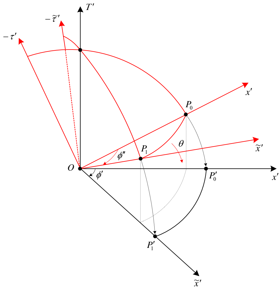
Fig. 2. Rotation of the \tau' - x' and \tilde{\tau}' - \tilde{x}' planes by \theta .
