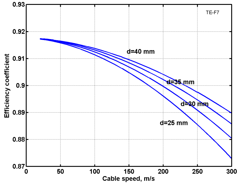
Fig. A5.7. Electric efficiency coefficient versus cable speed for cable diameter d = 25\text{--}40 mm, cable stress 6000\text{ kg/mm}^2 , cable length L = 7000 km, average cable altitude H = 10 km, aerodynamic efficiency of winged support devices k = 25 .
