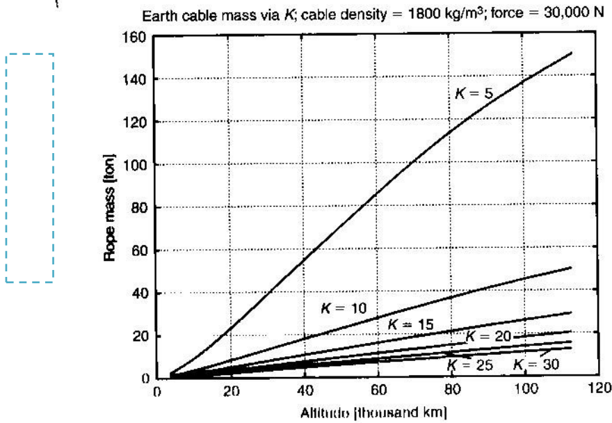
Fig. 1.9. Cable mass [tons] via counterweight altitude for Earth's surface force of 3 ton, cable density 1800 kg/m 3 , and K = 5-30 .
