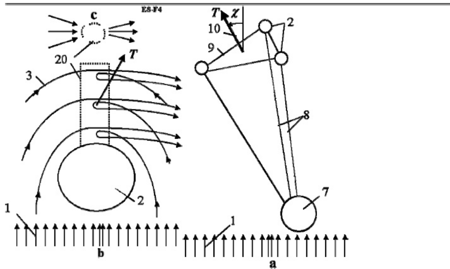
Figure 13.4. Two methods of controlling of the thrust direction: a – control using three balls. Notations are: 7 – spaceship (probe); 8 – links (cables) connected to the space ship and the electrostatic balls. 9 – cable connection of balls; 10 – T – thrust of the propulsion system; b – control of thrust direction by capacitor (electrostatic mirror). c – top view of capacitor. The other notations are presented in Figure 3a.
