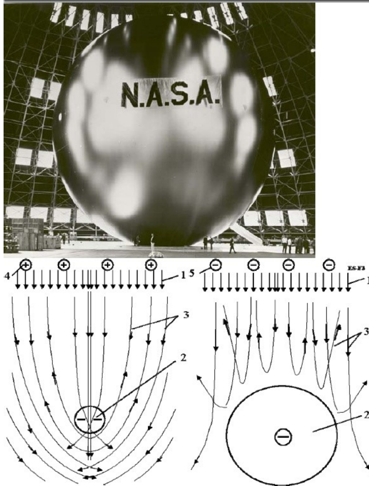
Figure 13.3b (up). A very large sphere, even of a thin film, can hold a massive charge. Here is an Echo balloon satellite of the early '60s, 30 meters (100 feet) across; note the men for scale. With suitable insulation and charge protection a very light sphere can hold enormous energies within. Credit: NASA. http://dayton.hq.nasa.gov/IMAGES/SMALL/GPN-2002-000203.jpg .
