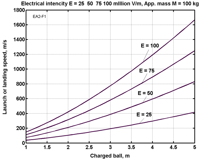
Fig. 14.8. Launch and landing (braking) speed of apparatus versus the charged ball radius and the electrical intensity (in million of volts/meter).
