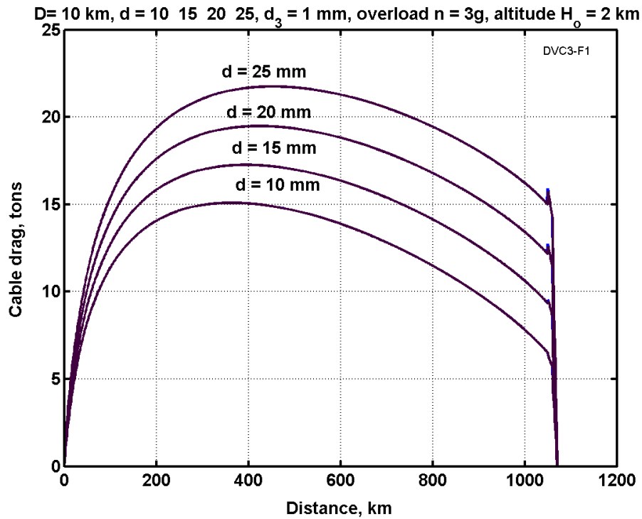
Fig. 2.9. Cable drag along the acceleration distance for initial cable diameter at ship d_0 = 10\text{--}25 \text{ mm} , cable diameter of part 3 d_3 = 1 \text{ mm} , overload 3g , at altitude 2 \text{ km} .
