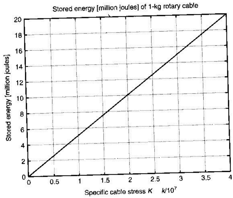
Fig. 3.16. Storage energy of 1 kg of the cable
