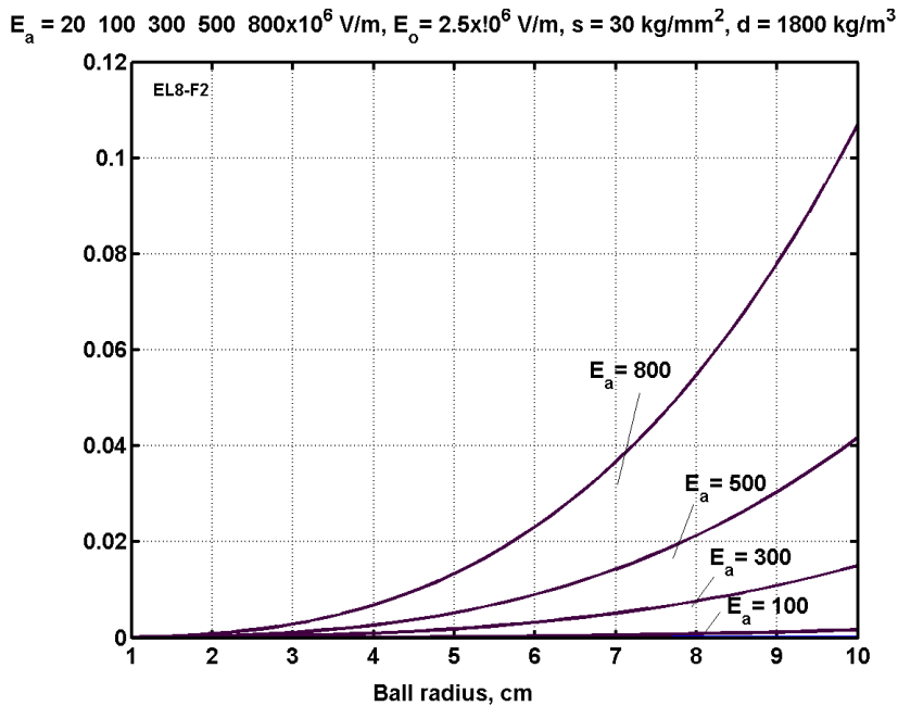
Fig. 15.7. Mass (kg) of small lifting ball versus radius of ball for the electrical intensity of the ball's surface E_a = (100-800) \times 10^6 \text{ V/m} , general electrical intensity E_o = 2.5 \times 10^6 \text{ V/m} , safe tensile stress of the ball cover 30 \text{ kg/mm}^2 , specific density of the ball cover 1800 \text{ kg/m}^3 .
