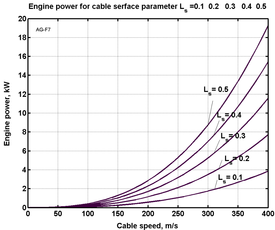
Fig. 9.7. Engine power versus cable speed for the cable surface parameter L_s = L^{0.8} s = 0.1-0.5 .
