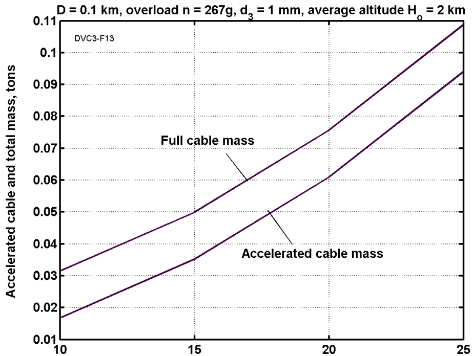
Fig. 2.13. Cable mass versus the initial cable diameter at ship 10–25 mm, for distance between drive stations L_1 = 0.1 km, overload n = 267g , d_3 = 1 mm, altitude H = 2 km.
