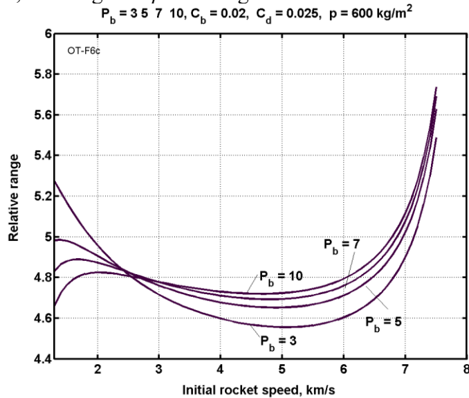
Fig. A4.16. Relative range of variable wing vehicle for the body drag coefficient C_b = 0.02 , the wing drag coefficient C_d = 0.025 , the wing load p = 600 \text{ kg/m}^2 , the body load P_b = 3-10 \text{ ton/m}^2 .
