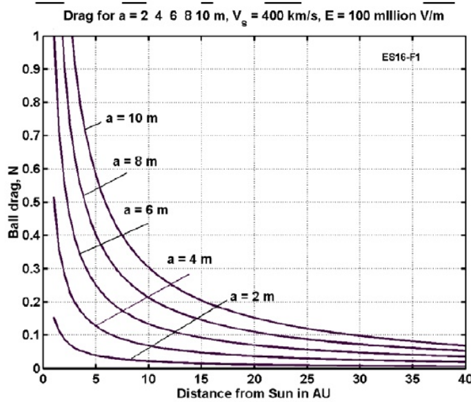
Figure 13.11. Drag of the electrostatic sail versus distance from the Sun (in AU) for ball radius a = 2-10 m, solar wind speed 400 km/s and electrical intensity E = 100 million volts/meter.
