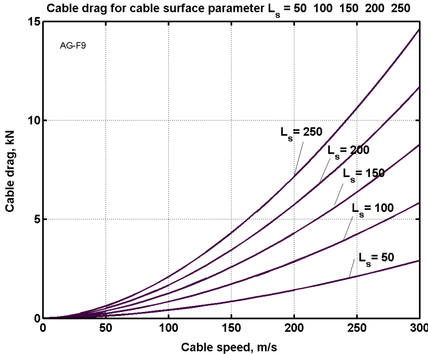
Fig. 9.9. Air cable drag versus cable speed for the cable surface parameter L_s = L^{0.8} s = 50\text{--}200 .
