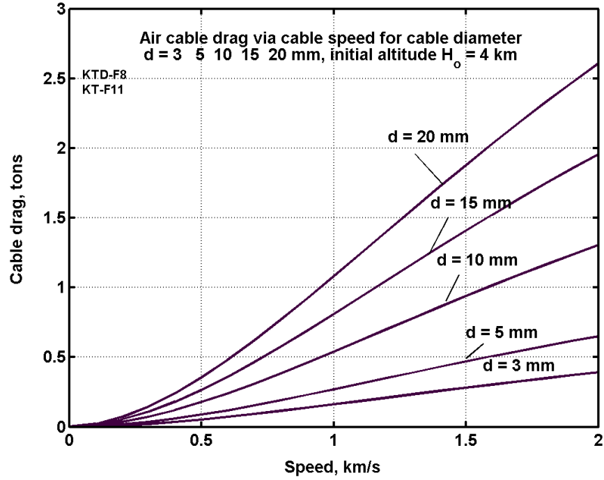
Fig. 5.11. Air cable drag via cable speed 0–2 km/s for different cable diameter.
