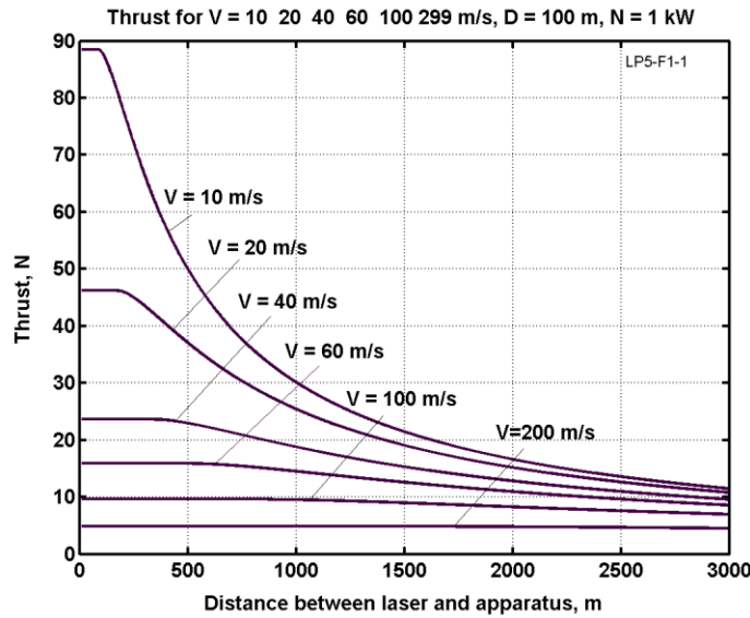
Fig. 12.7. Thrust (N) versus distance [m] for vehicle speed V = 10\text{--}200\ \text{m/s} , attenuation coefficient a = 0.5\ \text{dB} , cell size m = 30 , mirror diameter D = 100\ \text{m} , beam power N = 1\ \text{kW} .
