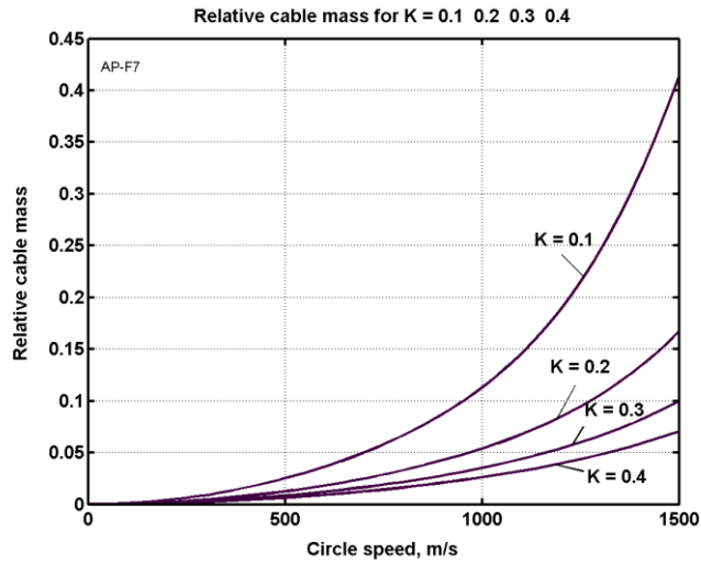
Fig. 11.7. Relative cable asteroid mass via circle speed in m/s and coefficient K = 0.1-0.4 .
