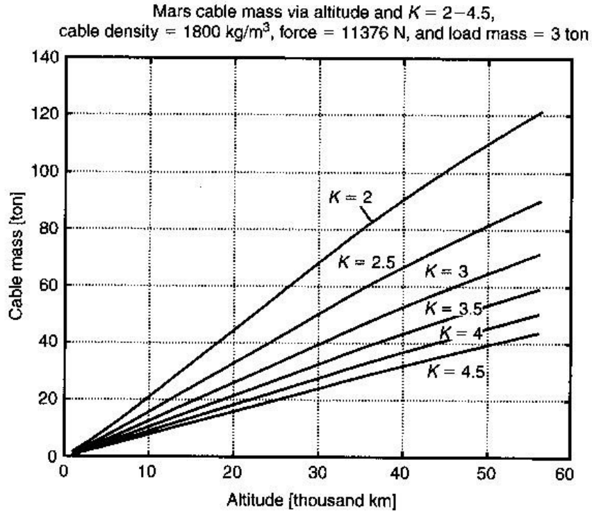
Fig. 1.24. Mars cable mass via altitude [thousand km], a cable density 1800 \text{ kg/m}^3 and a load mass of 3 ton.
