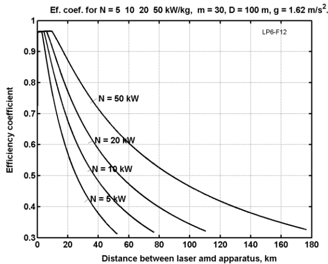
Fig. 12.10. Vertical launch of a space vehicle from the Earth's Moon (Moon gravity is g = 1.62 \text{ m/s}^2 ). Efficiency coefficient versus distance is computed for relative beam power N = 5\text{--}50 \text{ kW/kg} , attenuation coefficient a
