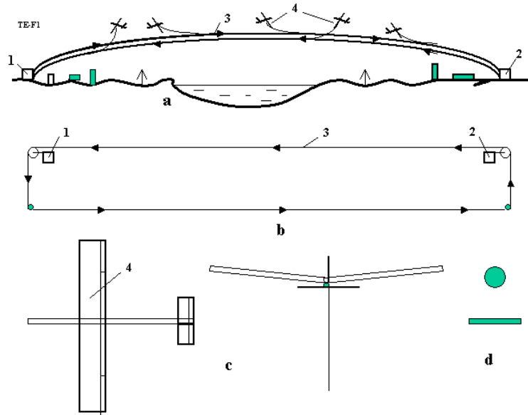
Fig. A5.1. Transferor of mechanical energy. Notations are: 1 – transmission station, 2 – reception station, 3 – closed-loop mobile cable, 4 – supporting winged device. a – transfer system (side view), b – transfer system (top view), c – supporting winged device, d – cross-section of the cable.
