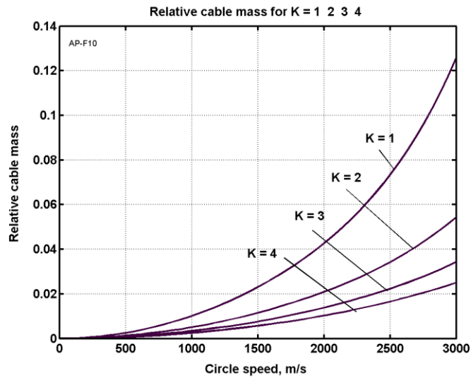
Fig. 11.10. Relative cable asteroid mass via circle speed in m/s and coefficient K = 1-4 .
