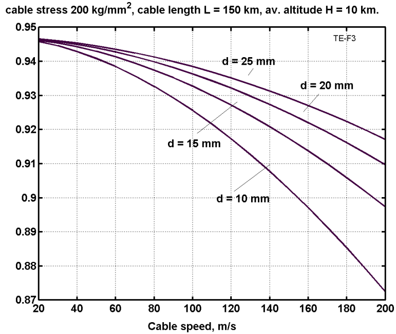
Fig. A5.3. Electrical efficiency coefficient versus cable speed for cable diameter d = 10\text{--}25 \text{ mm} , cable stress 200 \text{ kg/mm}^2 , cable length L = 150 \text{ km} , average cable altitude H = 10 \text{ km} , aerodynamic efficiency of winged support devices k = 25 .
