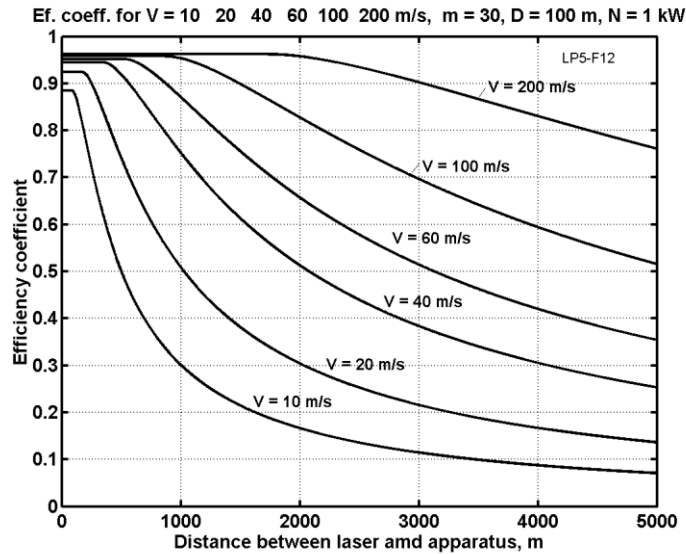
Fig. 12.8. Efficiency coefficient versus distance [m] for vehicle speed V = 10\text{--}200\ \text{m/s} , attenuation coefficient a = 0.5\ \text{dB} , cell size m = 30 , mirror diameter D = 100\ \text{m} , beam power N = 1\ \text{kW} .
