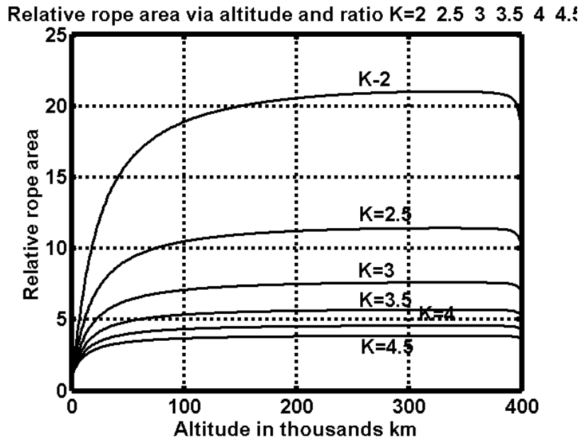
Fig. 7.2a. Relative area for a cable from Earth to Moon (up to 400,000 km) for stress coefficient K = 2 - 4.5 .
