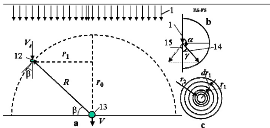
Figure 13.2. a - Interaction between solar wind and the electrostatic field of a charged ball. Notations are: 1 - solar wind (protons/electrons), 12 - charged particles (protons/electrons); 13 - electrically charged ball (balloon); 14 - line of turn of angle \gamma of a particle that is attracted (attracted force of unlike charges); 15 - line of turn of angle of a particle that is repelled (repulsive force of like charges); R - radius of interaction or neutral
