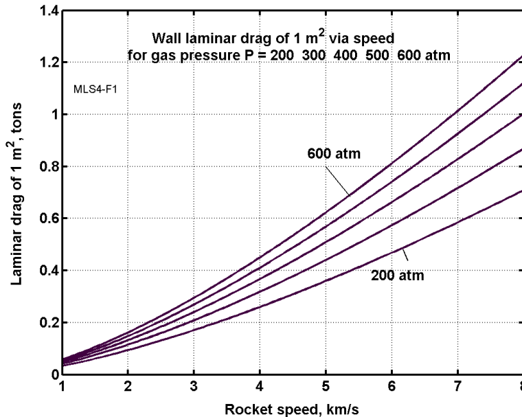
Fig. 6.13. Wall laminar drag of 1 m 2 versus speed for gas pressure 200–600 atm.
