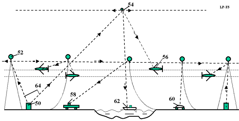
Fig. 12.4. Beam energy transfer to air, land, and sea vehicles. Notations are: 50 – beam energy station, 52 – control mirror suspended from a tethered air balloon, 54 – mirror suspended from planet satellite, 56 – aircraft, 58 – ground track, 60 – car, 62 – sea (ocean) ship, 64 – beams.
