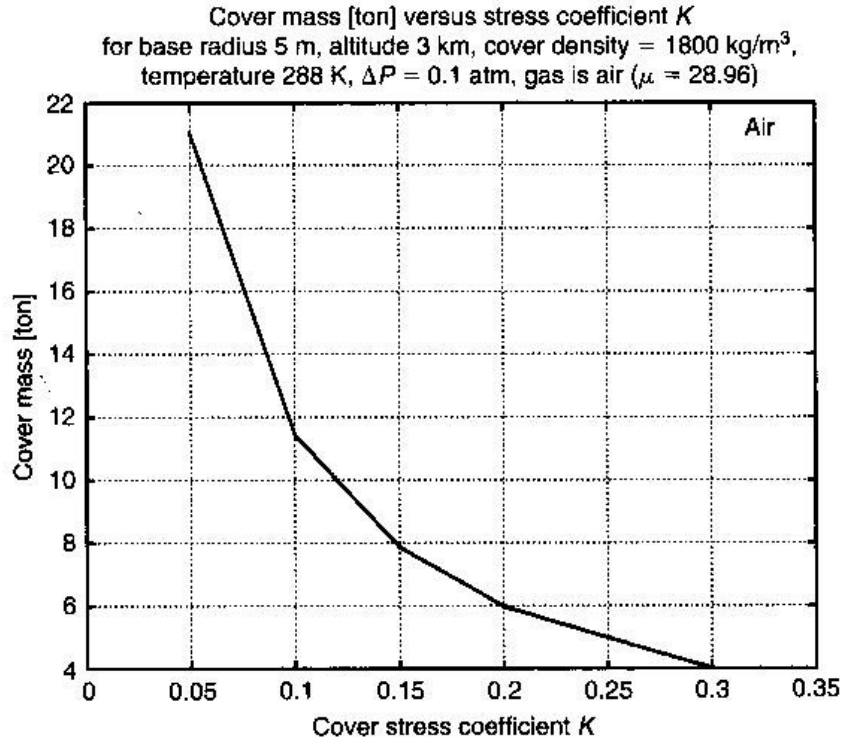
Fig. 4.9. Cover mass of the 3-km air tower versus stress coefficient.
