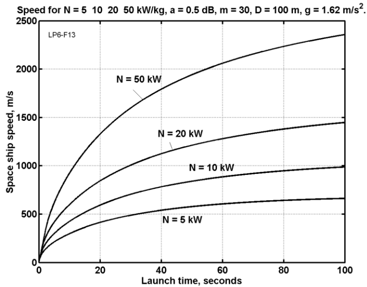
Fig. 12.11. Vertical launch of a space vehicle from the Earth's Moon (Moon gravity is g = 1.62 m/s 2 ). Space ship speed (m/s) versus time (seconds) is computed for relative beam power N = 5 – 50 kW/kg, attenuation coefficient a = 0.5 dB, cell size m = 30 , mirror diameter D = 100 m, \lambda = 1 micron.
