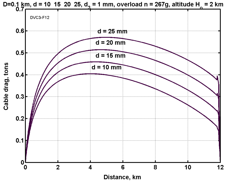
Fig. 2.12. Cable drag along the acceleration distance for initial cable diameter at ship d_o = 10-25 mm, cable diameter of part 3 d_3 = 1 mm, overload n = 267g , at altitude 2 km.
