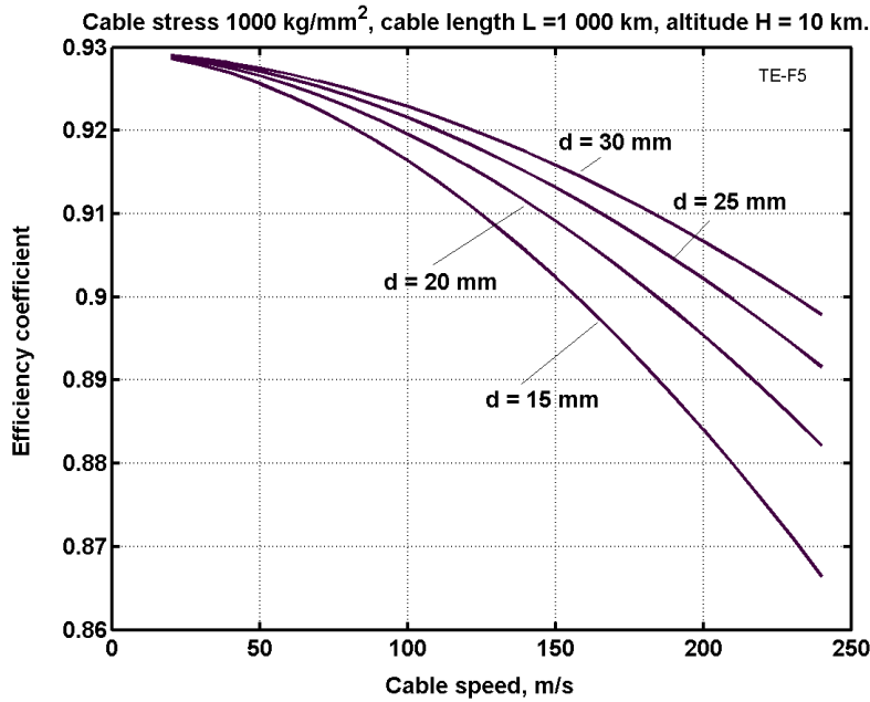
Fig. A5.5. Electric efficiency coefficient versus cable speed for cable diameter d = 15\text{--}30 \text{ mm} , cable stress 1000 \text{ kg/mm}^2 , cable length L = 1000 \text{ km} , average cable altitude H = 10 \text{ km} , aerodynamic efficiency of winged support devices k = 25 .
