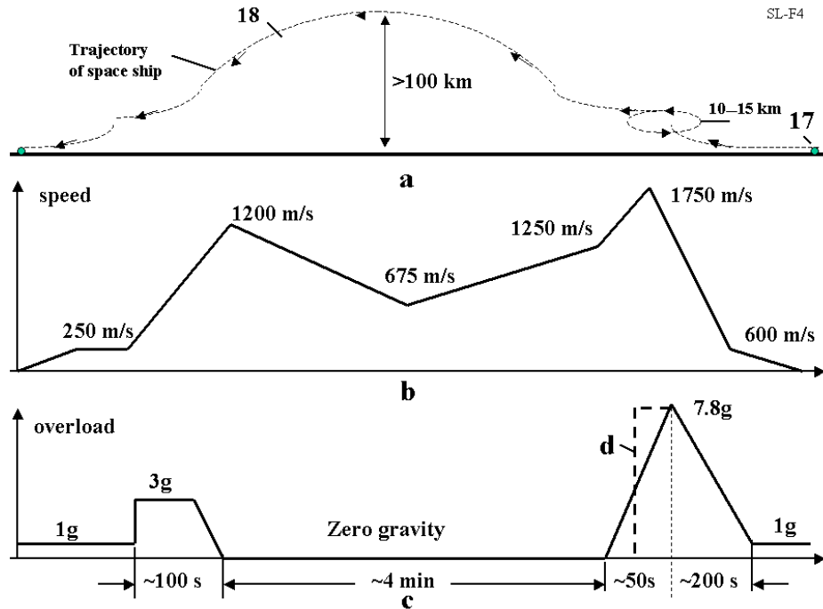
Fig. 10.4. a) Space flight trajectory. Notations: 17 – aircraft, 18 – trajectory of space ship. b) graph of ship speed (project 3). c) graph of ship overload (project 3). d) change of overload graph in project 4.
