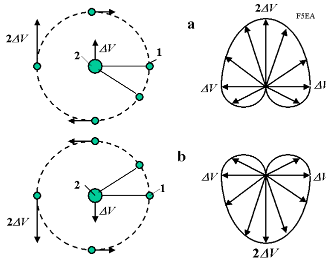
Fig. 11.4. Using the kinetic energy of an asteroid to change the space ship trajectory (speed and direction). On the right are cardioids of the additional velocity and its direction. The ship can get this velocity from the asteroid. Notations: 1 – space ship, 2 – asteroid, \Delta V – difference between velocities of space ship and asteroid. a) Case when the asteroid has the same direction as the ship; b) Case when the asteroid has the opposite direction to the ship a.
