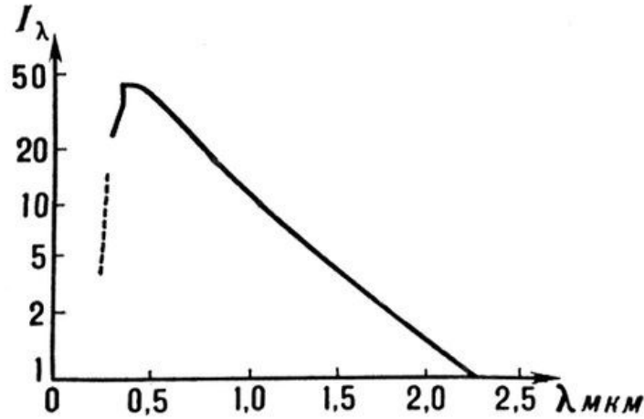
Fig. 18.4. Spectrum of solar radiation. \lambda is the wavelength [0–2.5 \mu\text{m} ], I_\lambda is the energy density.
