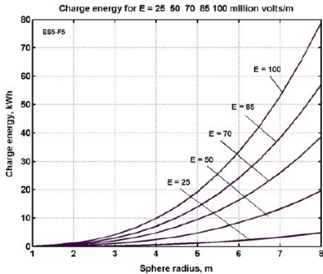
Figure 13.18. Initial expenditure of electrical energy needed to charge the space apparatus, a = 1 - 8 m, electrical intensity is 25–100 MV/m and coefficient of efficiency 1.
