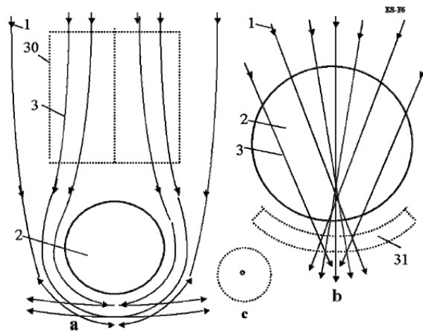
Figure 13.5. Two methods of decreasing the ball discharge: a – a charged cylindrical capacitor located in the front of the ball deflects particles from the ball; b – a capacitor located behind the ball adds speed to the particles and reflect the returned particles. c – top view of capacitor. Notations are: 30 –cylindrical capacitor, 31 – back capacitor (particles accelerator and electrostatic mirror)
