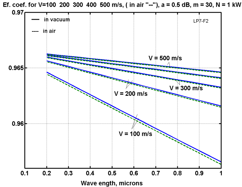
Fig. A3.8. Efficiency coefficient (equation (A3.7)) versus wavelength \lambda = 0.2 to 1 \mu\text{m} , a = 0.5 dB, m = 30 , N_0 = 1 kW, and rotor speed V = 100 to 500 m/s. The broken lines -- show the computations with air attenuation.
