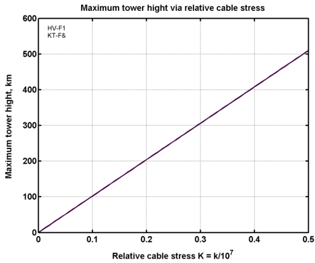
Fig. 5.7. Maximum tower height via relative cable stress.
