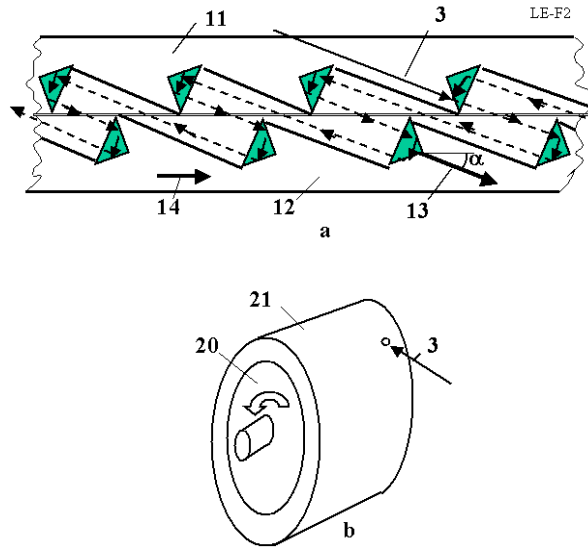
Fig. A3.2. Sloping reflective cells and light engine: a) 11 – stator (motionless), 12 – mobile rotor, 13 – local force (of single cell), 14 – direction of rotor movement; b) Light engine: 20 – rotor, 21 – stator.
