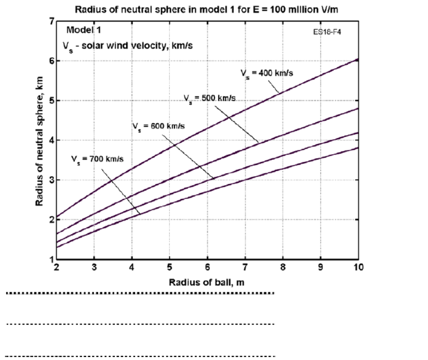
Figure 13.8. Radius of the neutral sphere in Model 1, when particle density in the sphere equals space plasma density.
