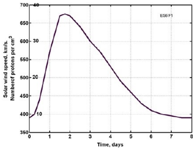
Figure 13.1a (up). Interaction of solar wind with Earth's magnetosphere. Figure 13.1b (down). Speed and density variations of solar wind in the Earth's orbit. The speed is in km/s, the density is in protons/cm 3 .
