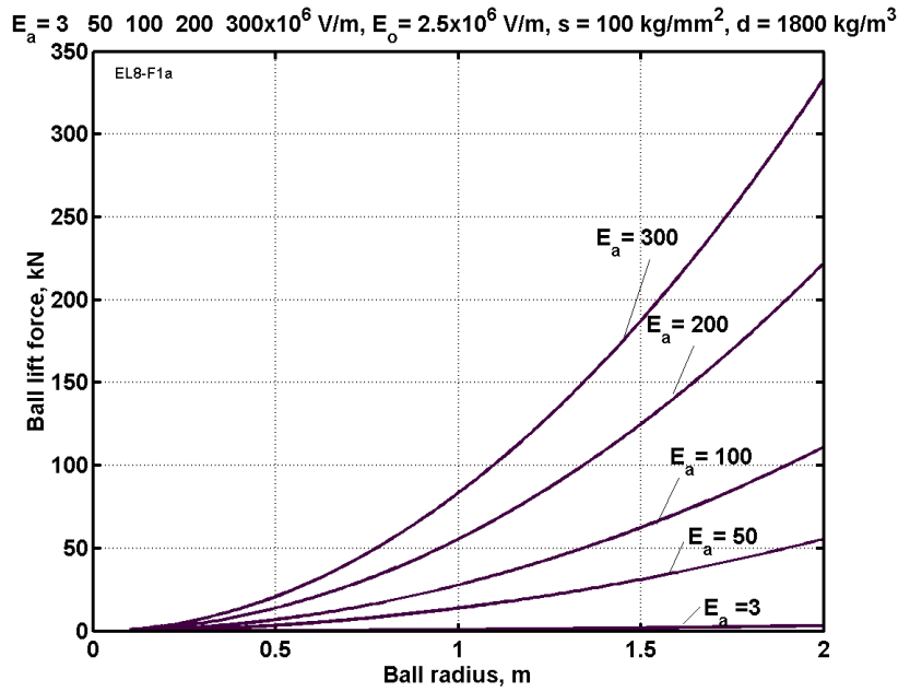
Fig. 15.8. Electrostatic lift force (kN) of the lifting ball versus radius of ball for the electrical intensity of the ball's surface E_a = (3-300) \times 10^6 \text{ V/m} , general electrical intensity E_o = 2.5 \times 10^6 \text{ V/m} , safe tensile stress of the ball cover 100 \text{ kg/mm}^2 , specific density of the ball cover 1800 \text{ kg/m}^3 .
