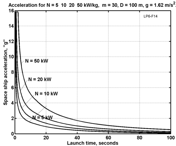
Fig. 12.12. Vertical launch of a space vehicle from the Earth's Moon (Moon gravity is g = 1.62 m/s 2 ). Limited ( <16g = 16 \times 9.81 = 157 m/s 2 ) acceleration is computed for relative beam power N = 5 – 50 kW/kg, attenuation coefficient a = 0.5 dB, cell size m = 30 , mirror diameter D = 100 m, \lambda = 1 micron.
