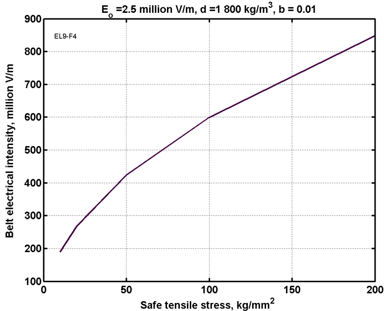
Fig. 15.11. Belt electrical intensity via safe tensile stress for general electrical intensity E_o = 2.5 \times 10^6 \text{ V/m} , safe tensile stress of the ball cover 10\text{--}200 \text{ kg/mm}^2 , \sigma = (10\text{--}200) \times 10^7 \text{ N/m}^2 ; \gamma – specific density of ball cover 1800 \text{ kg/m}^3 , relative thickness of belt cover, \delta = 0.01 \times a .
