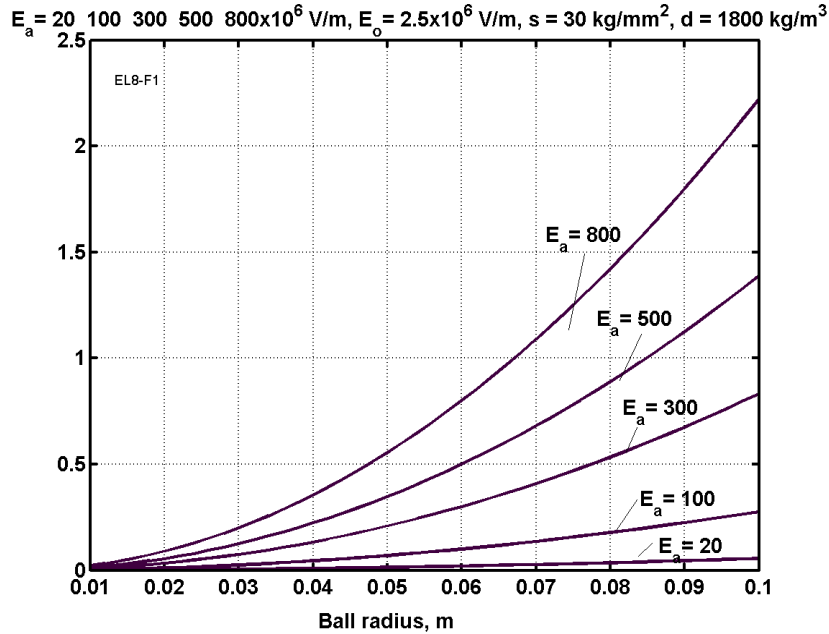
Fig. 15.6. Electrostatic lift force (kN) of small lifting ball versus radius of ball for the electrical intensity of the ball's surface E_a = (20-800) \times 10^6 \text{ V/m} , general electrical intensity E_o = 2.5 \times 10^6 \text{ V/m} , safe tensile stress of the ball cover 30 \text{ kg/mm}^2 , specific density of the ball cover 1800 \text{ kg/m}^3 .
