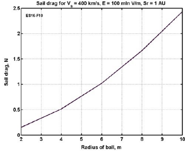
Figure 13.10. Drag of the electrostatic sail versus ball radius at the Earth's orbit (at 1 AU) for the solar wind speed 400 km/s and electrical intensity E = 100 million volts/meter.
