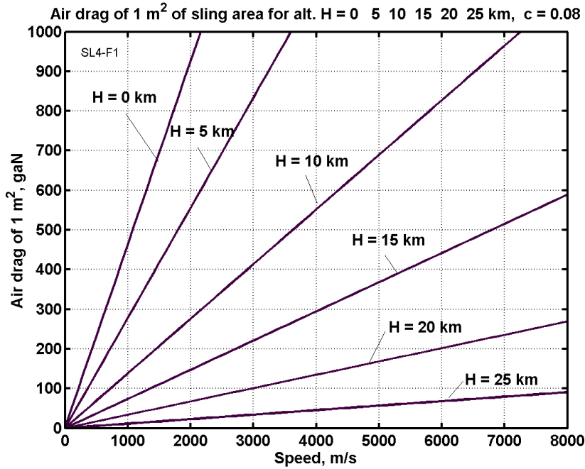
Fig. 10.7. Air drag of one square meter of wing sling (with relative profile thickness c = 0.08 ) based on speed and altitude [equation (10.3)].
