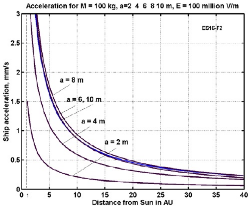
Figure 13.15 (down). Probe acceleration versus distance from the Sun and ball radius for useful probe mass M = 100 kg, and sail weight computed for safe cover stress \sigma = 180 kg/mm 2 , cover density \gamma = 1800 kg/m 3 , electric intensity E = 100 million volts/meter, at a distance from the Sun of 1 – 40 AU.
