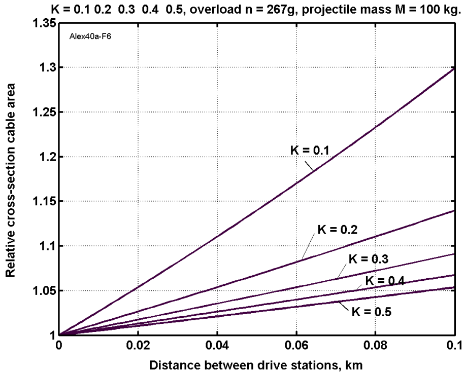
Fig. 2.6. Relative cable cross-sectional area versus the distance between drive stations for stress coefficient K = 0.1-0.5 ( K = 10^{-7}\sigma/\gamma ) and overload 267g , projectile mass 100 kg.
