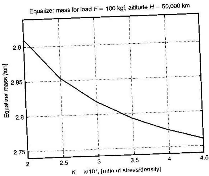
Fig. 1.27. Mars counterweight mass [tons] via the coefficient K = 2-4.5 for altitude 50,000 km ar
