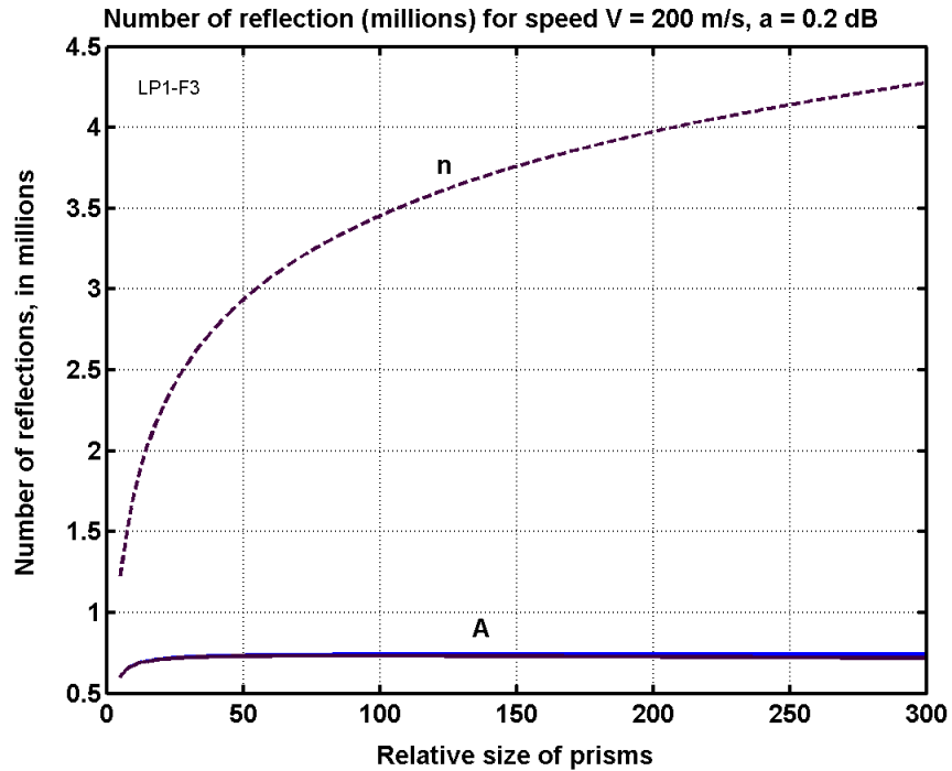
Fig. A3.5. Force coefficient, A (equation (A3.9)) and number of reflections n (equation (A3.6)) for rotor speed V = 200 m/s, a = 0.2 dB, and relative size of prisms m = 10-300 .
