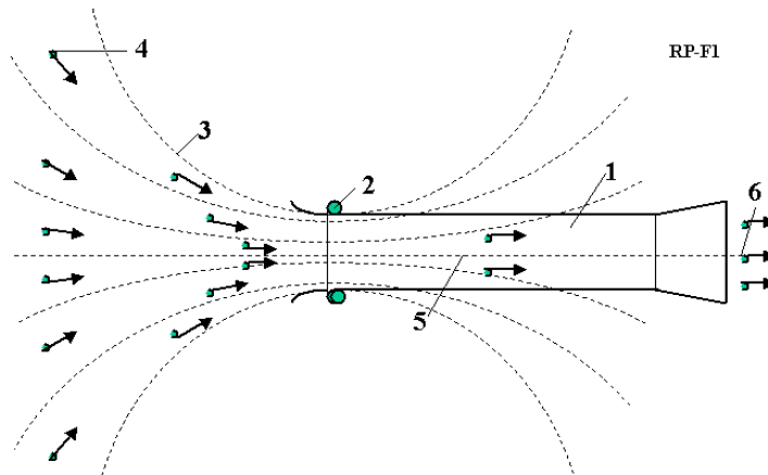
Fig. 19.1. Recombination space jet propulsion engine (actuator of magnetic field). Notations are: 1 engine, 2 – solenoid, 3 – magnetic lines, 4 – charged particles, 5 – recombination zone, 6 – exit.
