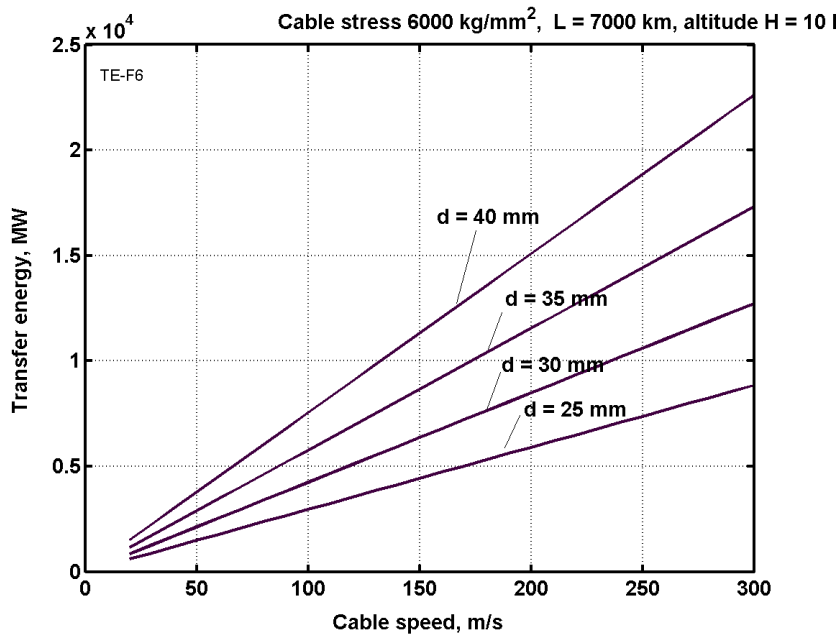
Fig.A5.6. Transfer energy versus cable speed for cable diameter d = 25\text{--}40 \text{ mm} , cable stress 6000 \text{ kg/mm}^2 , cable length L = 7000 \text{ km} , average cable altitude H = 10 \text{ km} , aerodynamic efficiency of winged support devices k = 25 .
