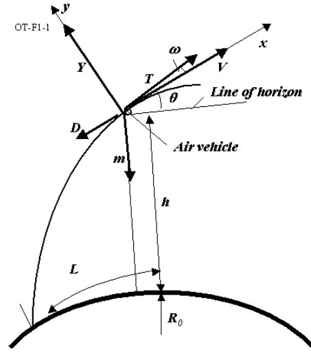
Fig. A4.1 Vehicle forces and coordinate system.
