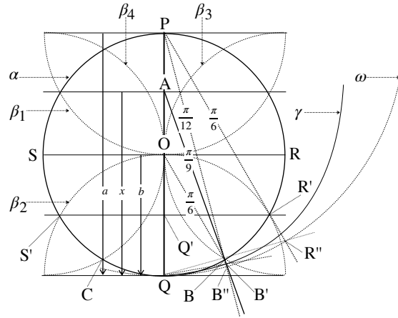
Fig.7 Proof model of trisection of angles
