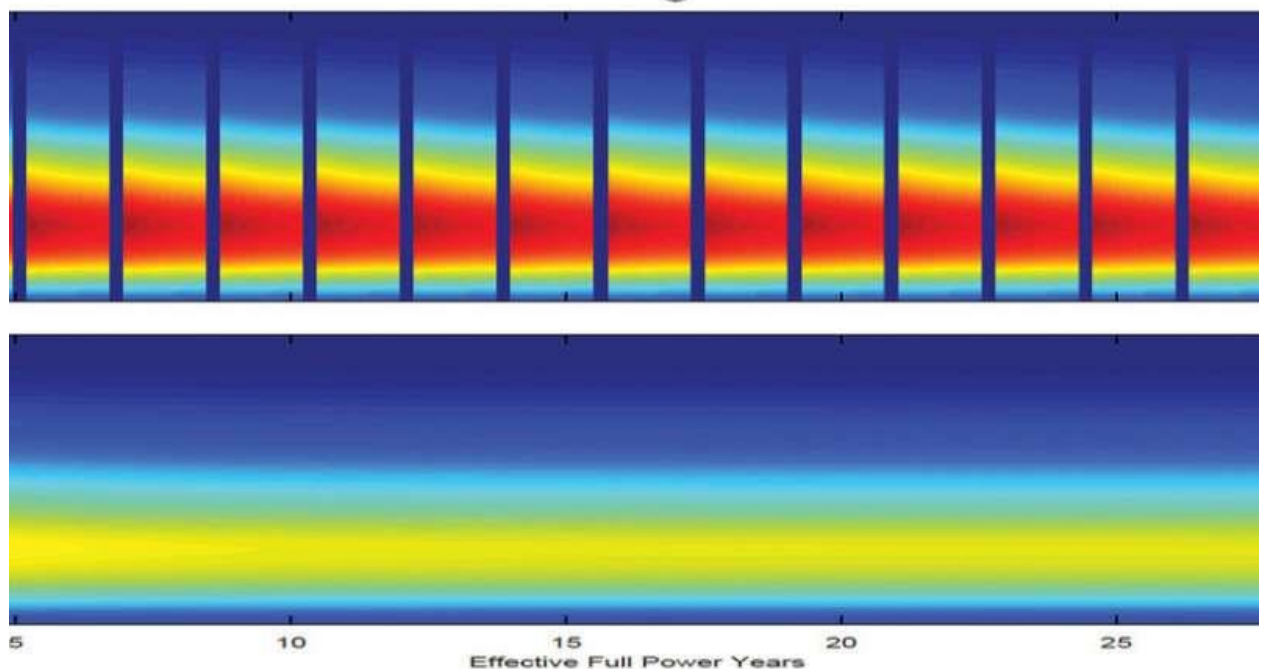
These images compare the evolution of antineutrino spectrum and antineutrino detector response as a function of reactor operational time in a pressurized water reactor and an ultra-long cycle fast reactor. Credit: Georgia Tech
