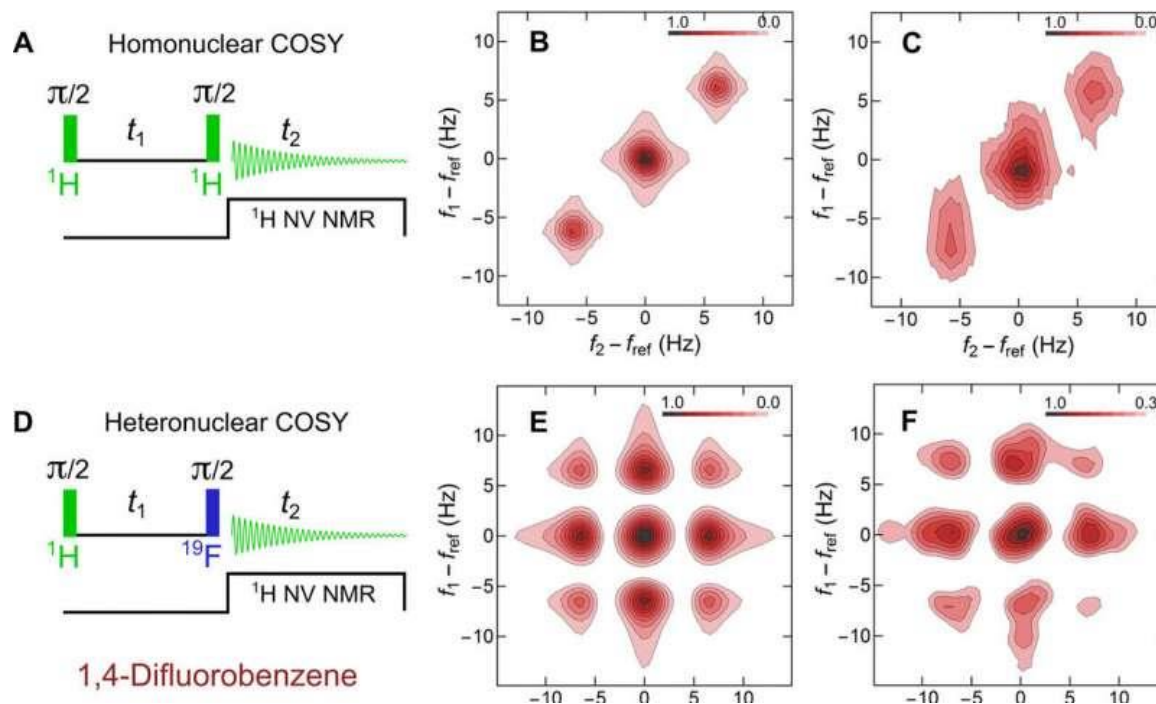
2D COSY NMR of DFB. (A) Homonuclear COSY pulse sequence, (B) simulated spectrum, and (C) experimental NV NMR spectrum of DFB. (D) A modified heteronuclear COSY sequence reveals off-diagonal peaks in both (E) simulation and (F) experiment. Color scales correspond to the normalized absolute value of the 2D Fourier transform. Vertical axes ( f_1 - f_{ref} ) correspond to the frequencies of the t_1 dimension, and horizontal axes ( f_2 - f_{ref} ) correspond to the frequencies of the t_2 dimension. In (C), 14 values of t_1 in 0.021-s increments up to 0.294 s were used. Total acquisition time was 22 hours. In (F), 16 values of t_1 in 0.021-s increments up to 0.336 s were used. Total acquisition time was 25 hours. In both cases, the t_2 acquisition spanned from 0 to 1.25 s. All simulations were performed using the SPINACH package. Simulation and experimental data use the same windowing functions. Credit: Science Advances, doi: 10.1126/sciadv.aaw7895.
