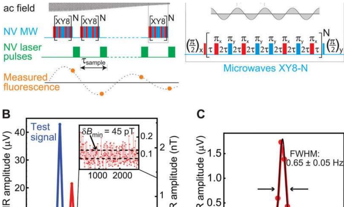
Characterization of pre-polarized NV NMR. (A) The synchronized readout pulse sequence. It consists of a train of XY8-N pulses that perform successive phase measurements of the ac magnetic field produced by processing nuclei. The measured fluorescence reflects an aliased version of the nuclear ac field projection. The entire sequence is repeated every 2.5 to 4.25 s (1.25 s for flow and the remainder for detection). (B) NV NMR spectra (absolute value of Fourier transform) of water (red) and an applied 2.5-nT amplitude test field (blue) for an effective acquisition time of 5.2 s (average of 60 traces; total measurement time, 150 s). The NMR signal amplitude obtained from the processed photodetector signal is recorded in \mu\text{V} . The conversion to magnetic field amplitude
