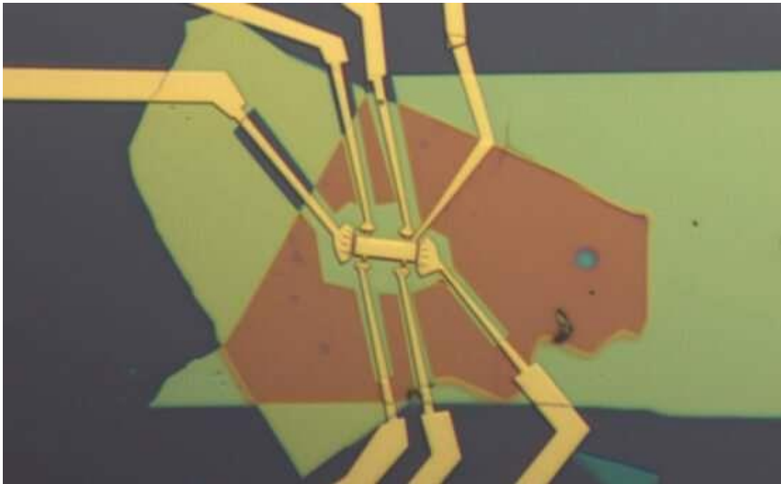
Optical micrograph of the assembled stacked structure, which consists of two graphene sheets sandwiched between two protective layers made of hexagonal boron nitride. Credit: Aaron Sharpe
