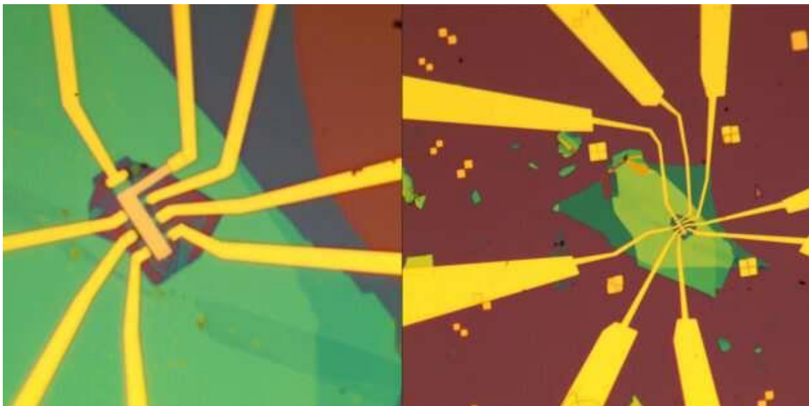
Two views of the trilayer graphene/boron nitride heterostructure device as seen through an optical microscope. The gold, nanofabricated electric contacts are shown in yellow; the silicon dioxide/silicon substrate is shown in brown; and the boron nitride flakes are shown in green. The
