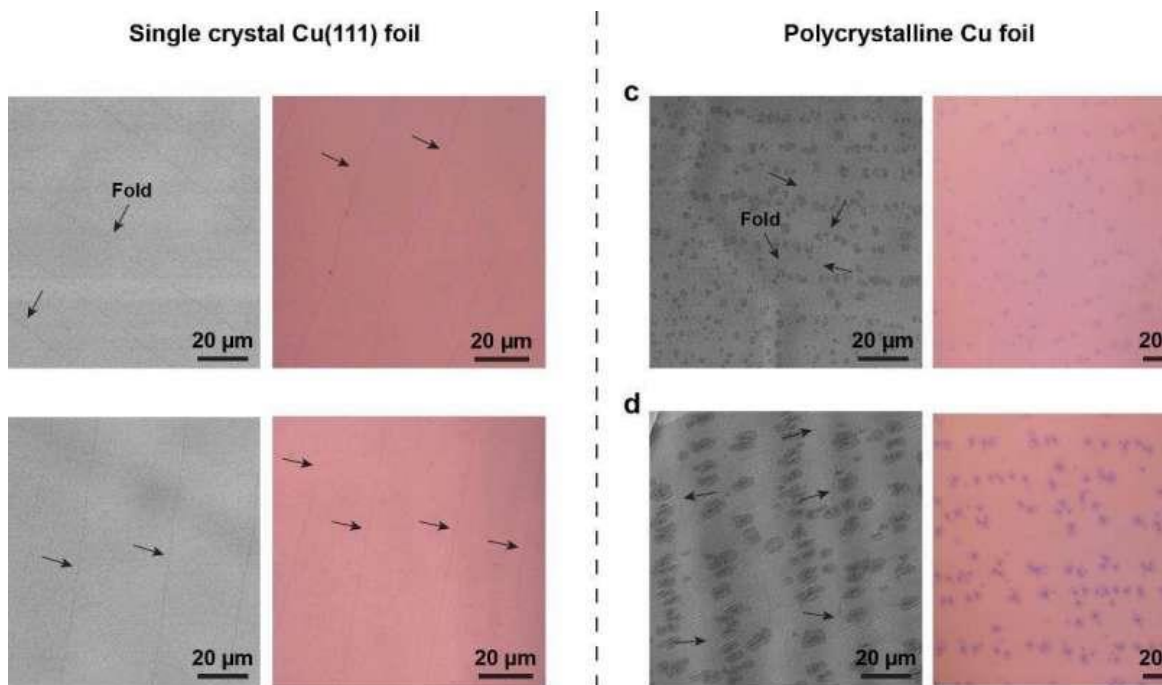
Figure 3 (a-b) (left panel) SEM images of adlayer-free single crystal graphene films on Cu(111) foils and (right panel) optical images of the films after transfer to 300 nm SiO 2 /Si wafers. (c-d) (left panel) SEM images of polycrystalline graphene films with adlayers on polycrystalline Cu foils and (right panel) optical images of the films after transfer to 300 nm SiO 2 /Si wafers. CVD parameters for gas flow and pressure were as follows: (a, c) H 2 /CH 4 (200 sccm / 1 sccm) at 2.0 Torr; (b, d) H 2 /CH 4 (30 sccm / 30 sccm 0.1% CH 4 in Ar) at 30.0 Torr. The black arrows point to folds. Credit: Institute for Basic Science
