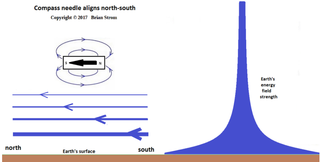
Figure 3. A compass needle in the Earth's magnetic field.
